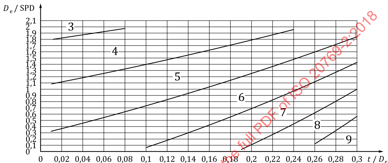
Figure 6 — Minimum number of DWSI exposures circumferentially around a pipe, as a function of the ratios t / D_e and D_e / SPD , where SPD is the distance from the source to the pipe axis (centre)
