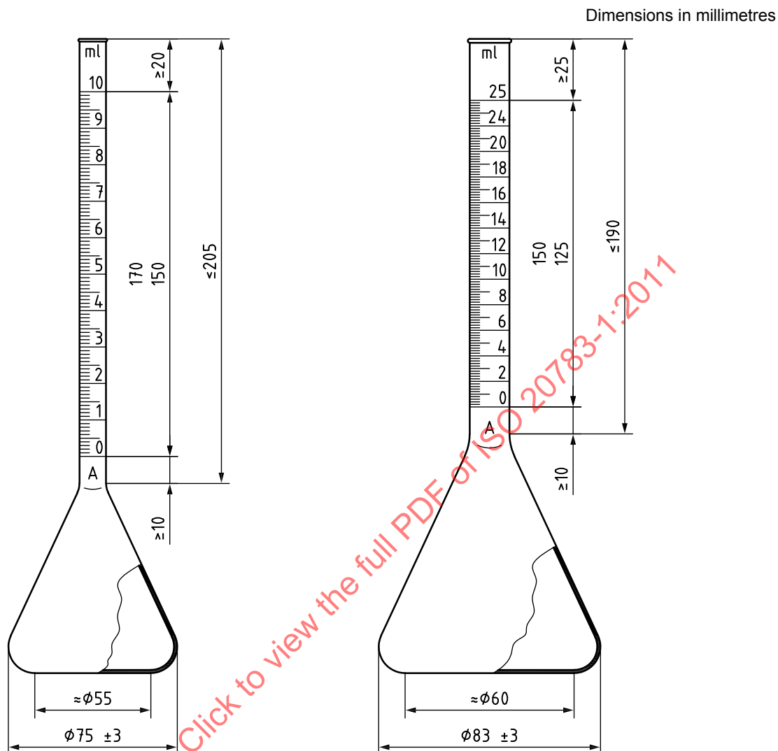
Figure 1 — Hirschsohn flasks
