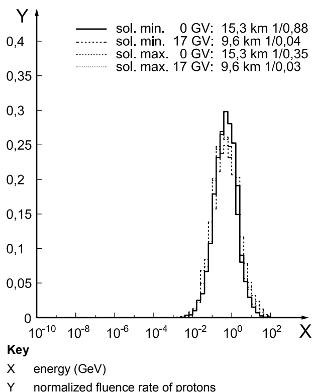
Figure A.2 — Normalized energy distribution of proton fluence rate
