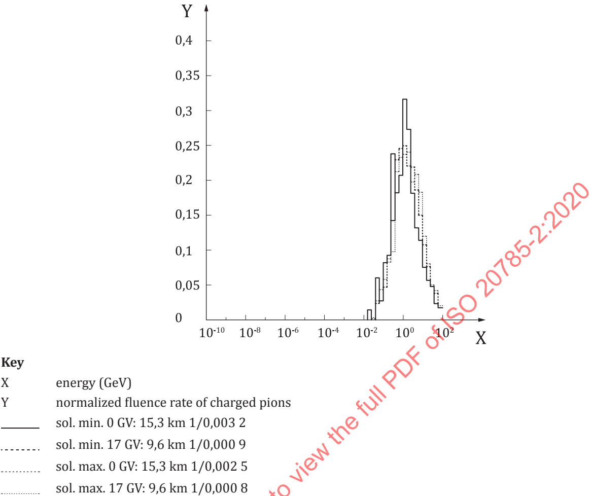
Figure A.3 — Normalized energy distribution of fluence rate of charged pions
