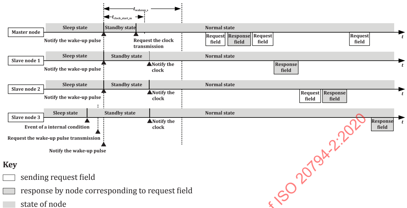
Figure 8 — Master node clock transmission timing
