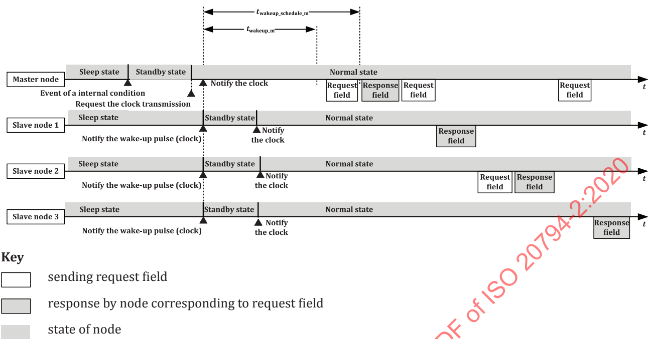
Figure 7 — Wake-up sequence of master node trigger
