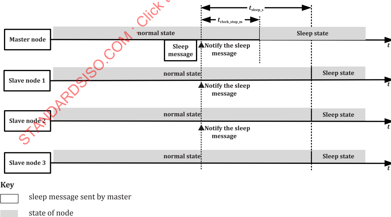
Figure 16 — Slave node receives sleep message
