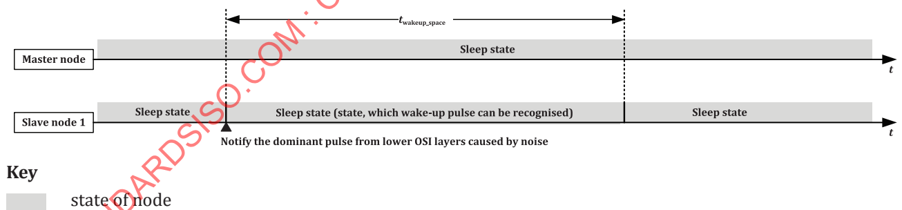
Figure 13 — Sleep sequence of no clock after dominant pulse received
