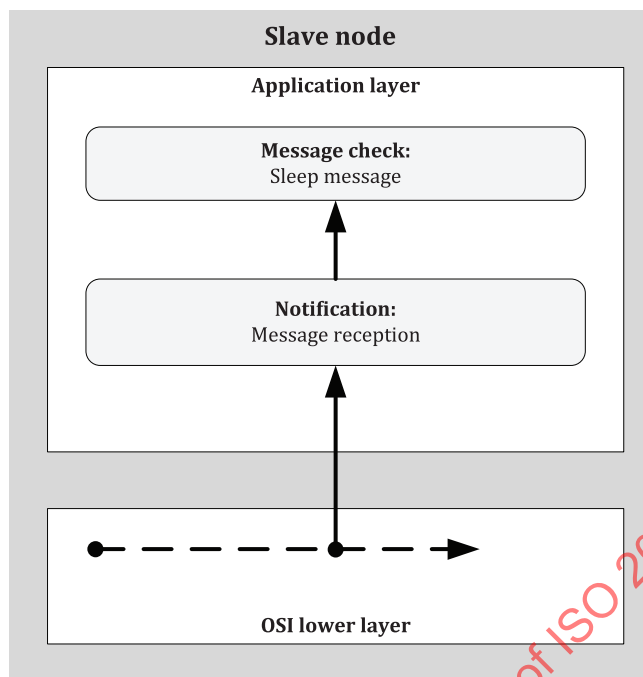
Figure 15 — Slave node sleep message
