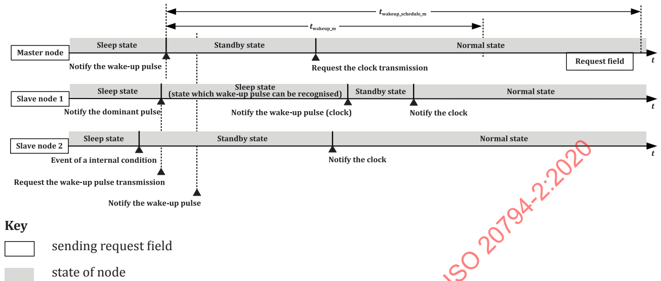
Figure 12 — Wake-up sequence by dominant pulse and clock notification
