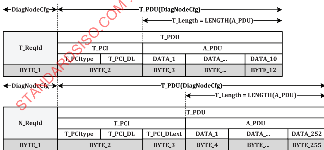
Figure 5 — TL T_Data.req and T_Data.ind with T_Ptype = DiagNodeCfg
