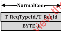
Figure 3 — TL T_Data.req and T_Data.ind with T_Ptype = NormalCom (T_Length = NULL)
