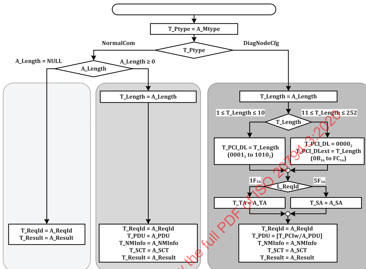
Figure 7 — TL transmission logic
