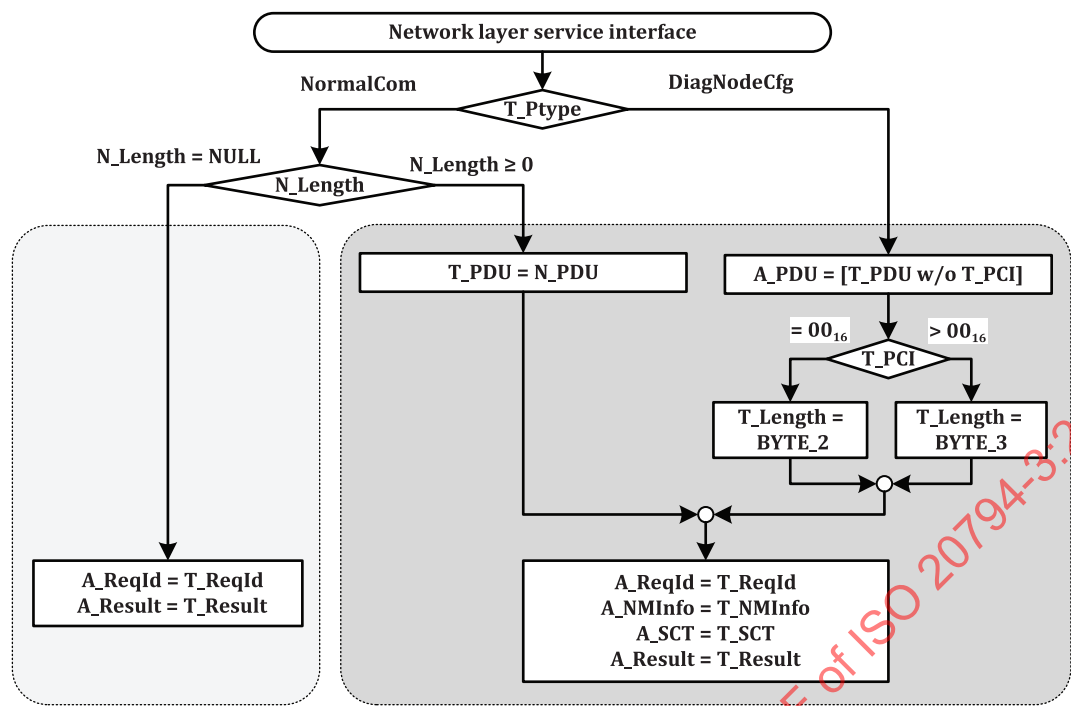
Figure 8 — TL reception function model
