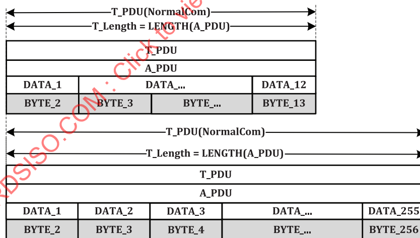
Figure 4 — TL T_Data.req and T_Data.ind with T_Ptype = NormalCom (T_Length ≥ '0')
