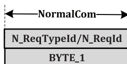
Figure 10 — NL N_Data.req and N_Data.ind with N_Ptype = NormalCom (N_Length = NULL)
