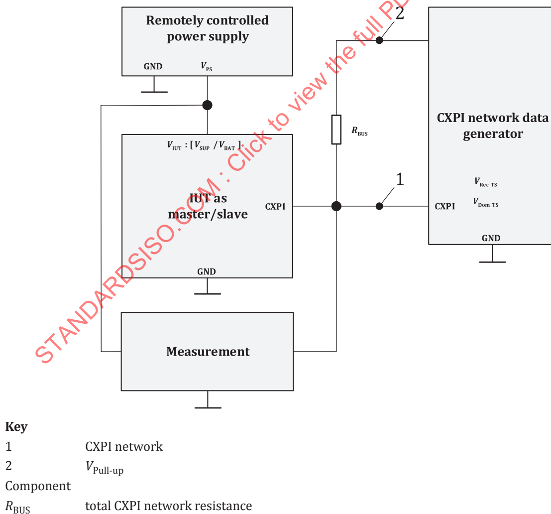
Figure 47 — Test system – Operating voltage range test set-up
