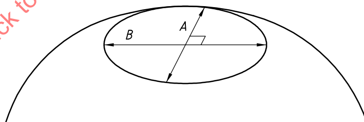
Figure 1 — Wear scar on ball specimen
