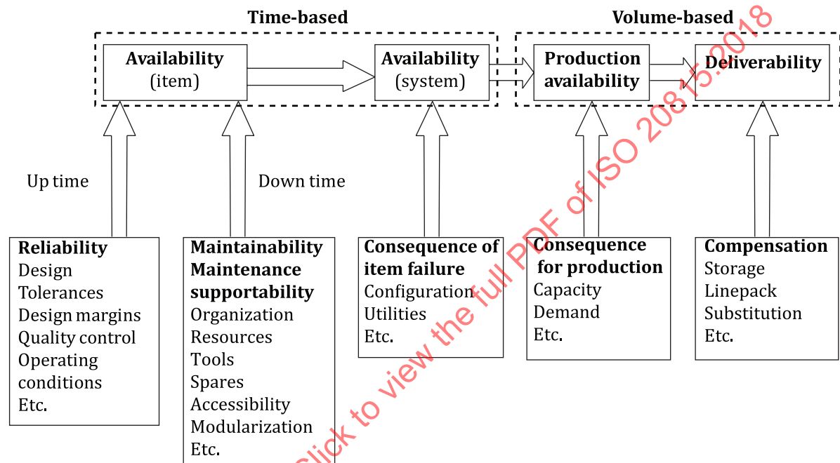
Figure G.1 — Illustration of the relationship between some time-based and volume-based production assurance terms
