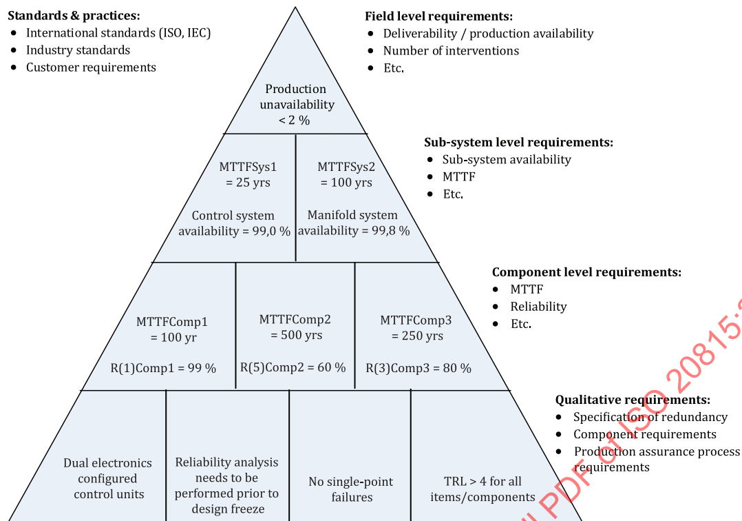
Figure F.1 — Typical reliability requirements — Subsea application example
