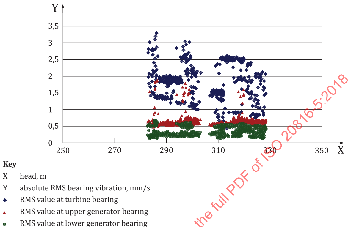
Figure B.2 — Example of bearing housing vibration in turbine operation of a pump-turbine
