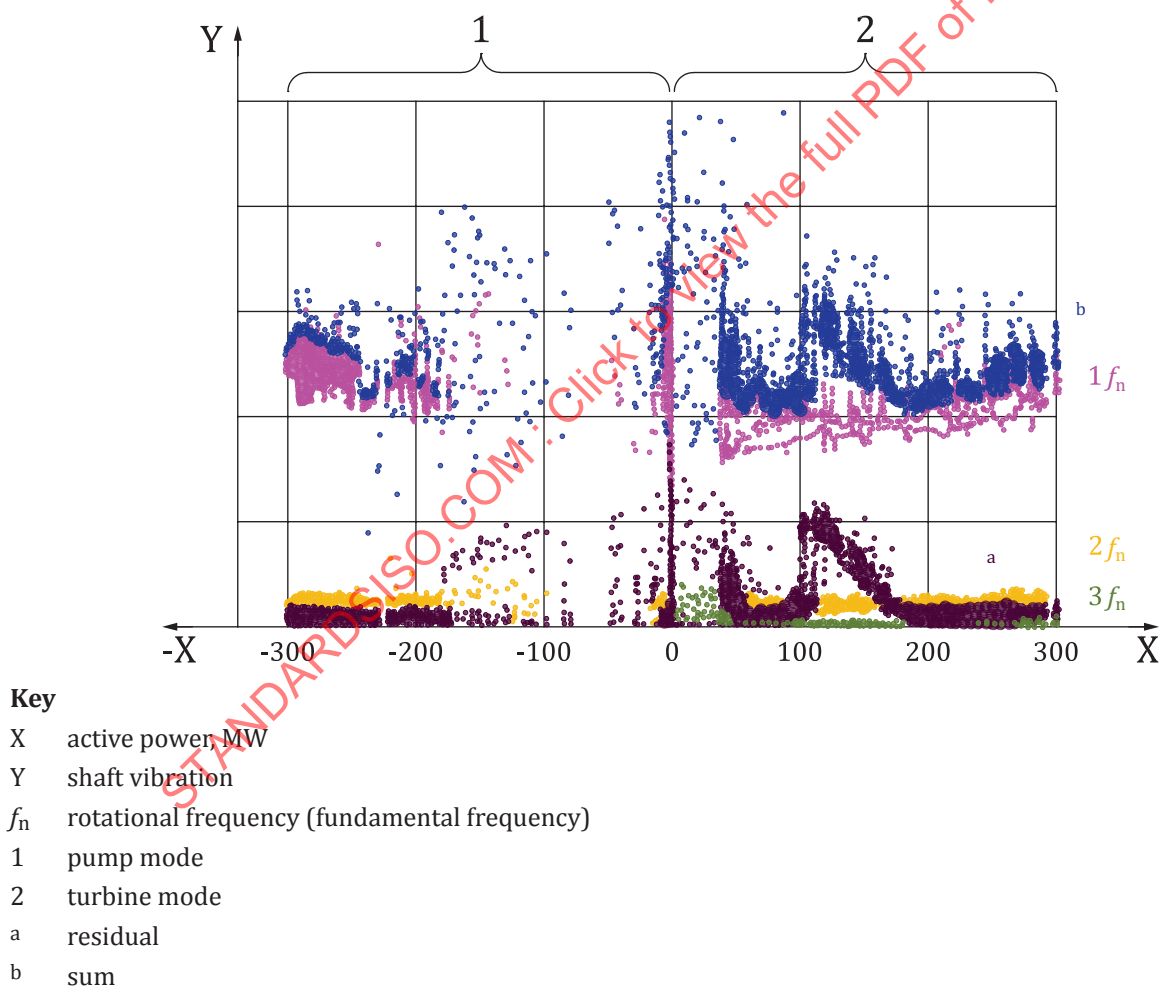
Figure B.1 — Example of individual shaft vibration components of a pump-turbine, the residual and the sum
