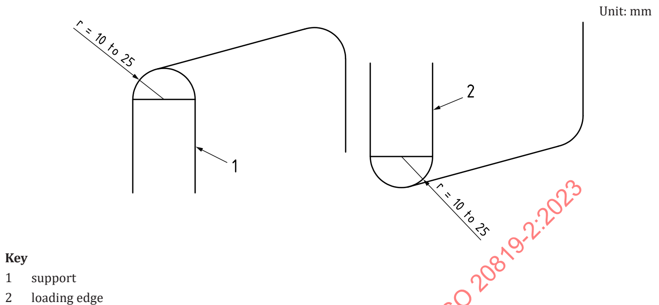
Figure 1 — Example of support and loading edge
