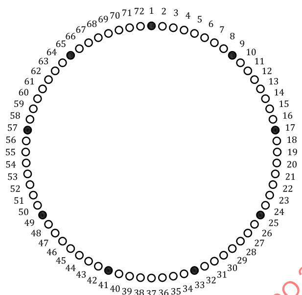
r) 72 well rotor – 9 sensors
