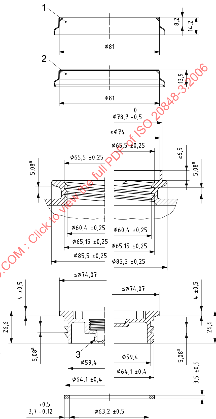
Figure E.2 — Plug/bung closure system BCS G2 × 5
