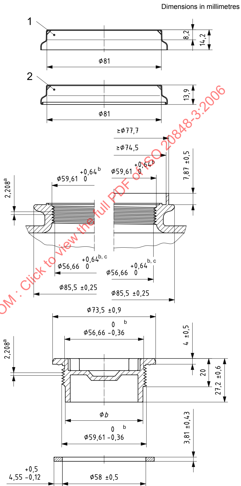
Figure F.2 — Plug/bung closure system BCS G2 × 11,5
