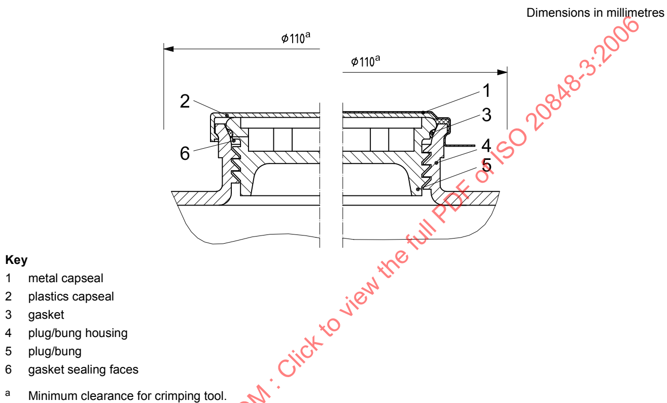
Figure B.1 — Plug/bung closure system BCS 56 × 4 — general view
