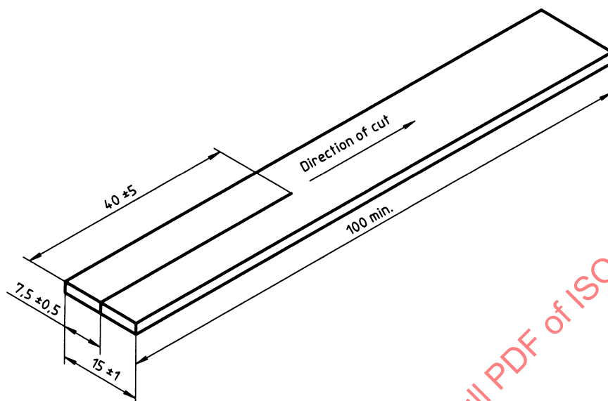
Figure 1 - Trousers test piece
