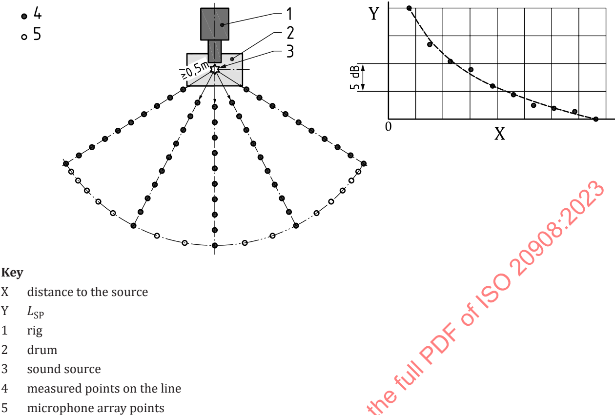
Figure 6 — Example of validation according to 6.5.2 for circular array setup
