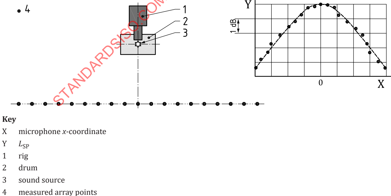
Figure 9 — Example of validation according to 6.5.4 for linear array
