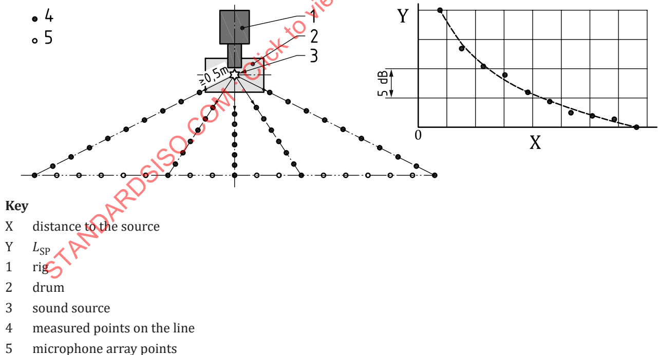
Figure 5 — Example of validation according to 6.5.2 for linear array setup
