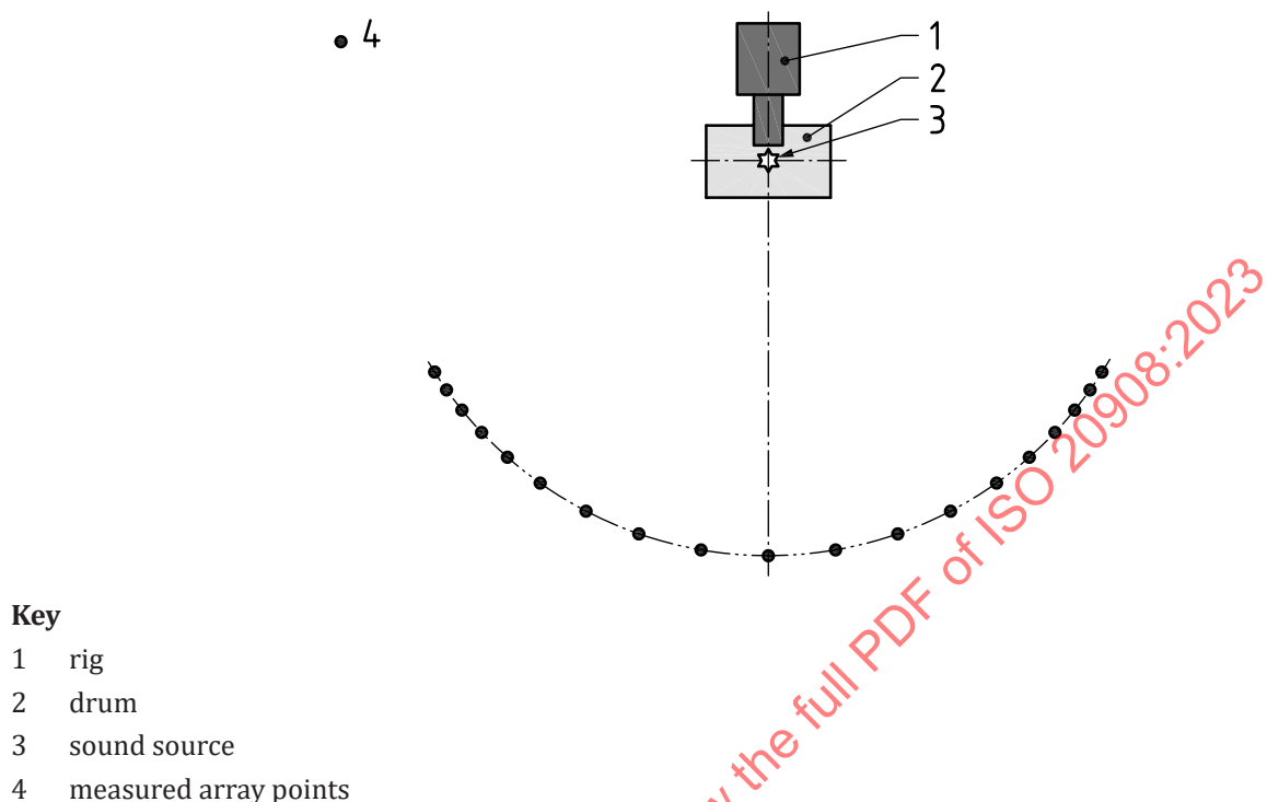
Figure 10 — Example of validation according to 6.5.4 for circular array
