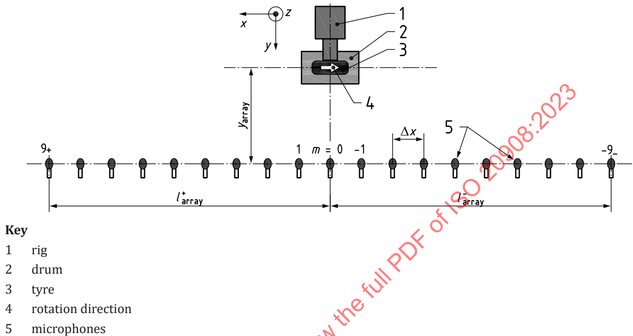
Figure 2 — Linear microphone array setup
