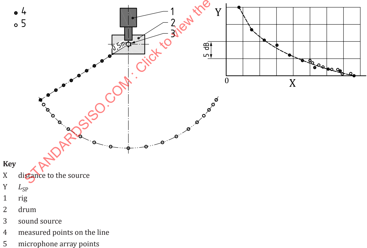
Figure 8 — Example of validation according to 6.5.3 for circular array setup
