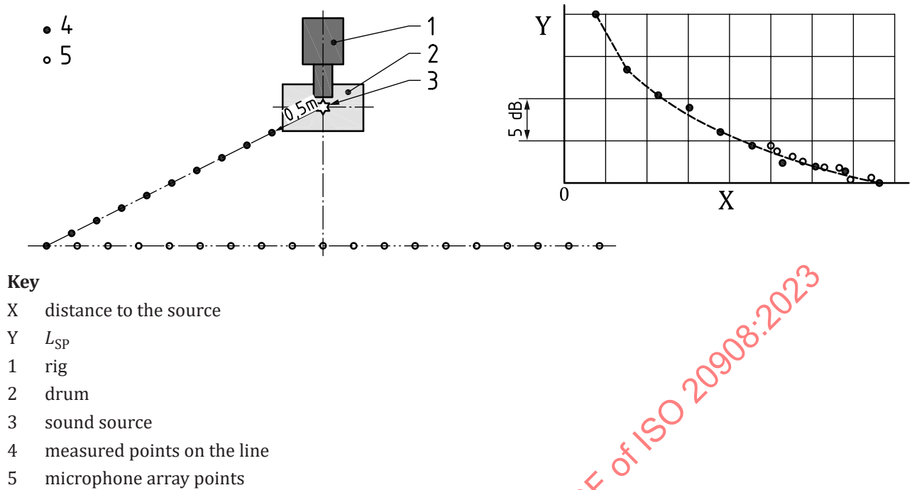
Figure 7 — Example of validation according to 6.5.3 for linear array setup
