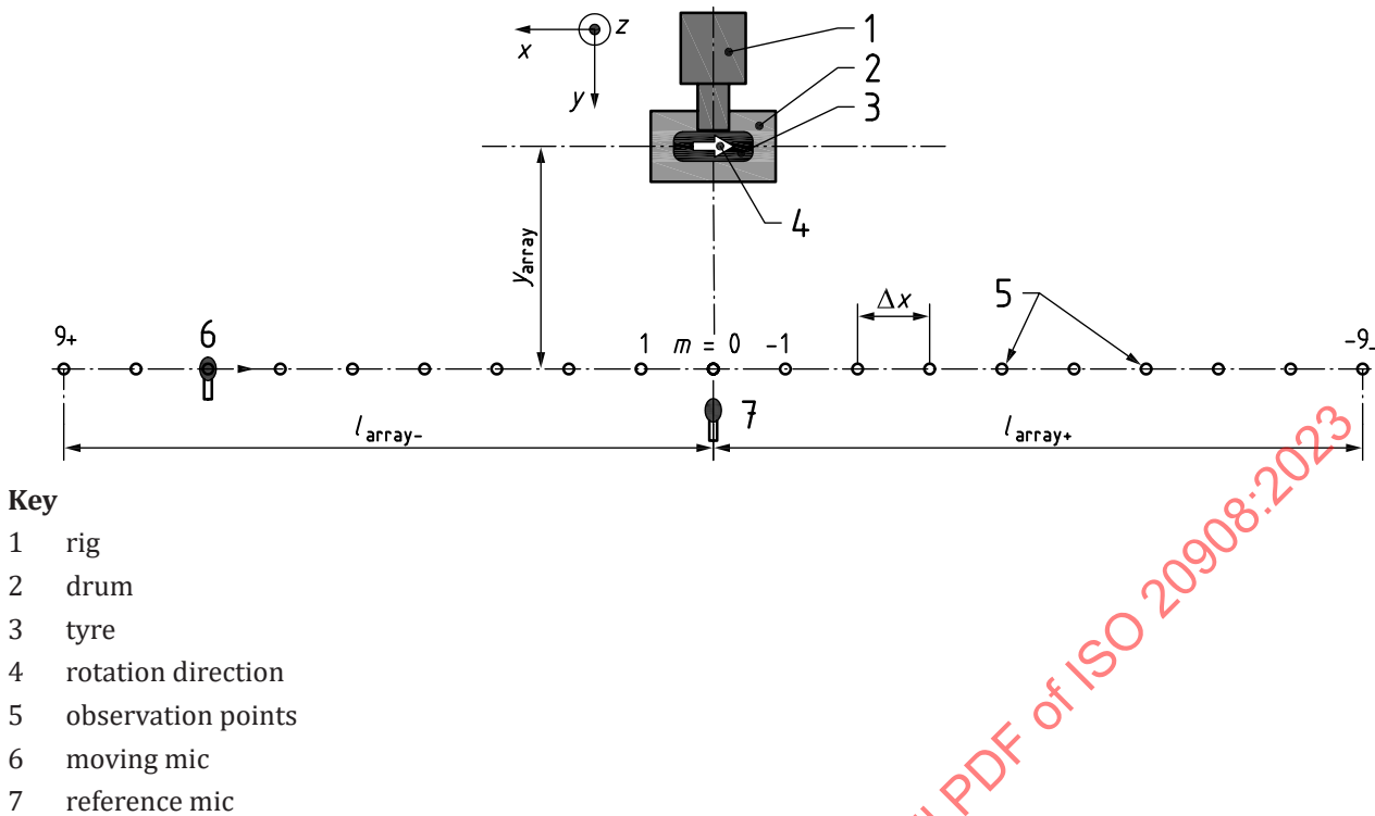
Figure 4 — One microphone measurement set up
