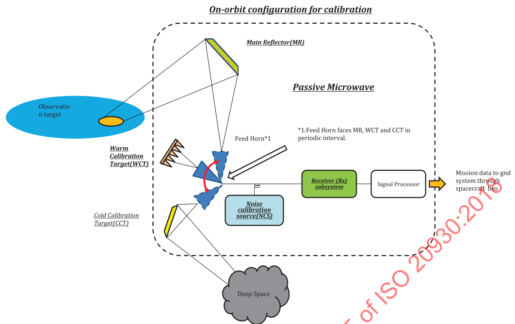
Figure A.3 — On-orbit configuration
