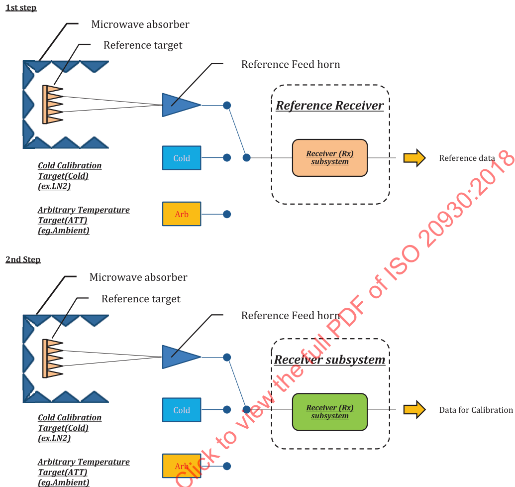
Figure A.1 — Ground test configuration image for Rx sub-system or receiver
