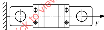
Figure 2 — Pull-test
