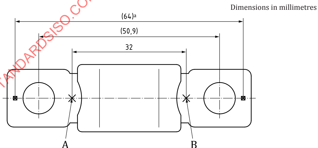
Figure 3 — Measurement points SF36-70V
