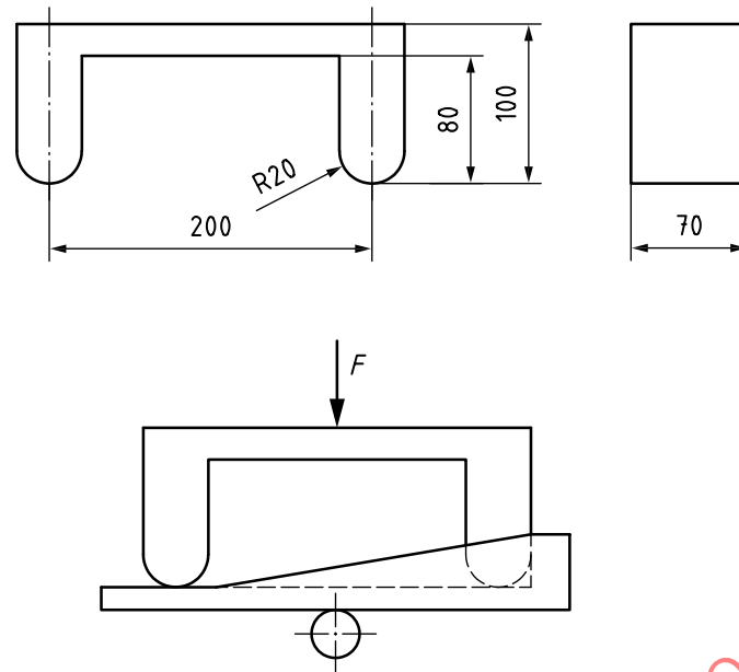
Figure 3 — Test device for testing foot supports
