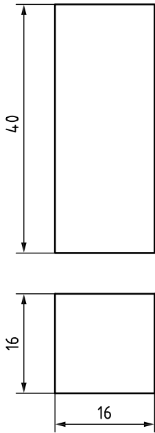
Figure 4 — Schematic of type I specimen
