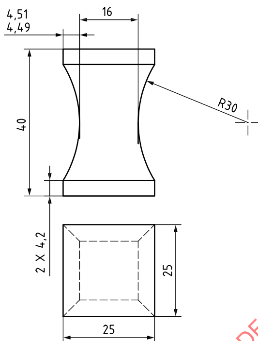
Figure 5 — Schematic of type II specimen
