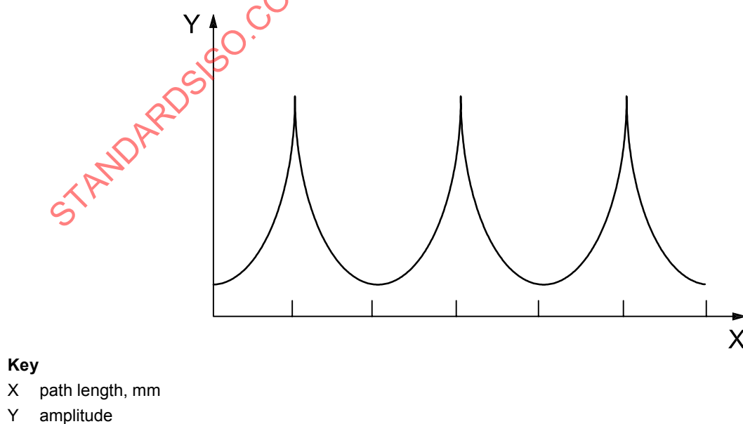
Figure A.1 — Constructive and destructive interference for continuous wave excitation
