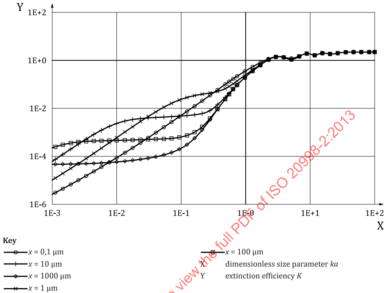
Figure C.1 — Typical extinction function for spherical glass particles in water Reference [29]
