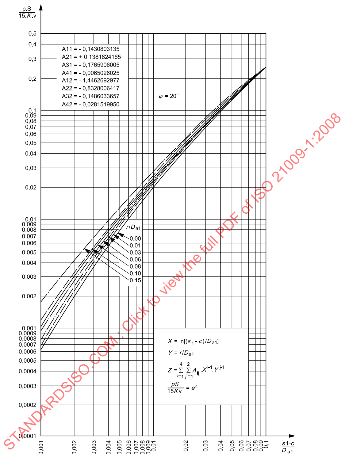
Figure 10.2 — Permissible value, \frac{pS}{15KV} , for convergent cone with an opening angle \varphi = 20^\circ
