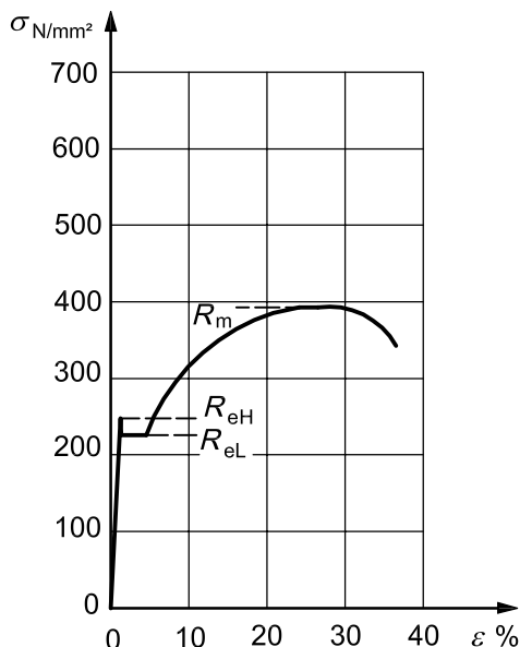
Figure C.1 — Stress/strain curve for carbon steel
