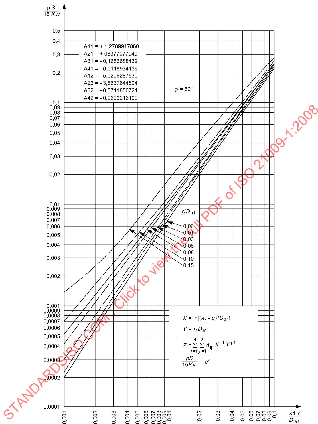
Figure 10.5 — Permissible value, \frac{pS}{15Kv} , for convergent cone with an opening angle \varphi = 50^\circ
