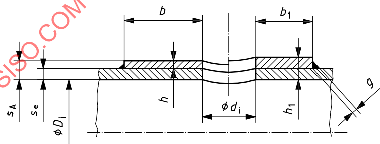
Figure 18 — Pad reinforcement
