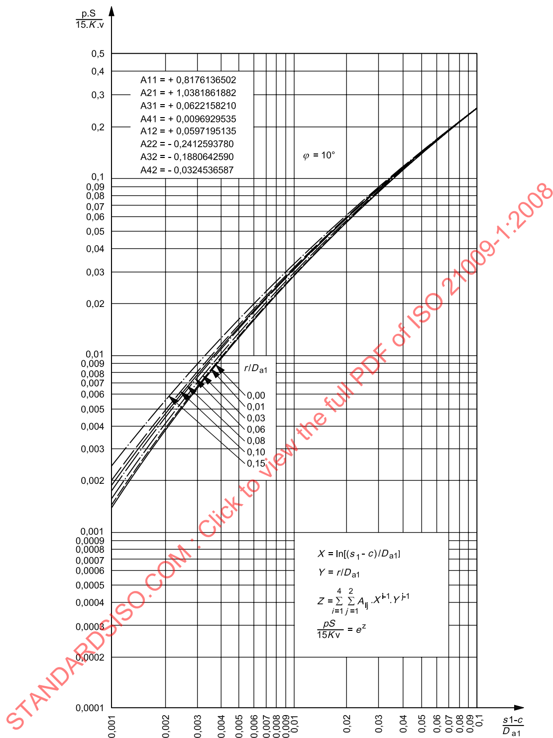
Figure 10.1 — Permissible value, \frac{pS}{15Kv} , for convergent cone with an opening angle \varphi = 10^\circ
