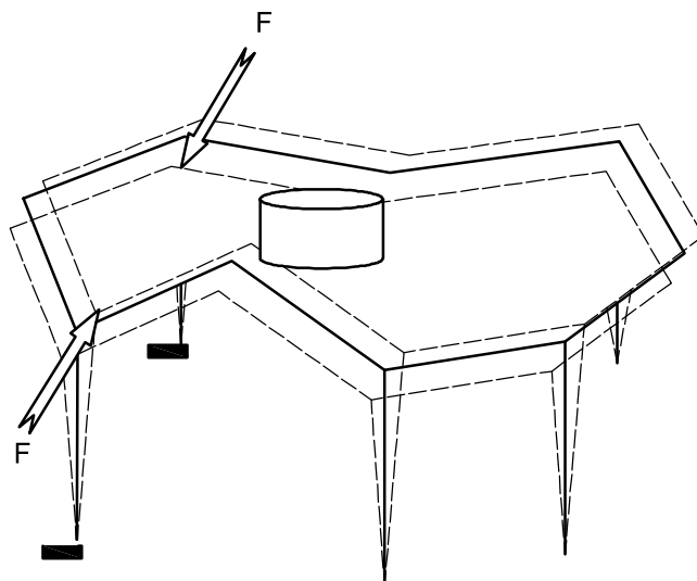
Figure 5 — Strength under horizontal static force test — Irregularly shaped table — Third and fourth directions
