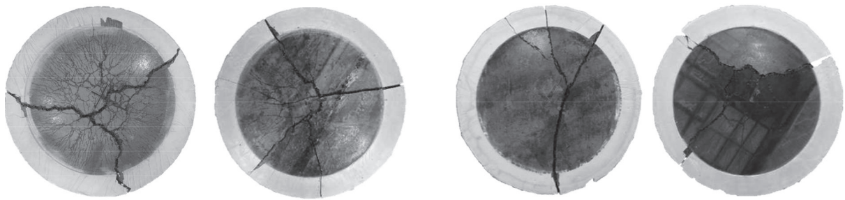
a) Fracture origin inside the loading ring — High energy b) Fracture origin outside the loading ring — Low energy
