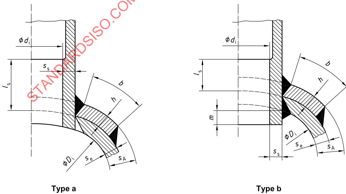
Figure 21 — Pad
