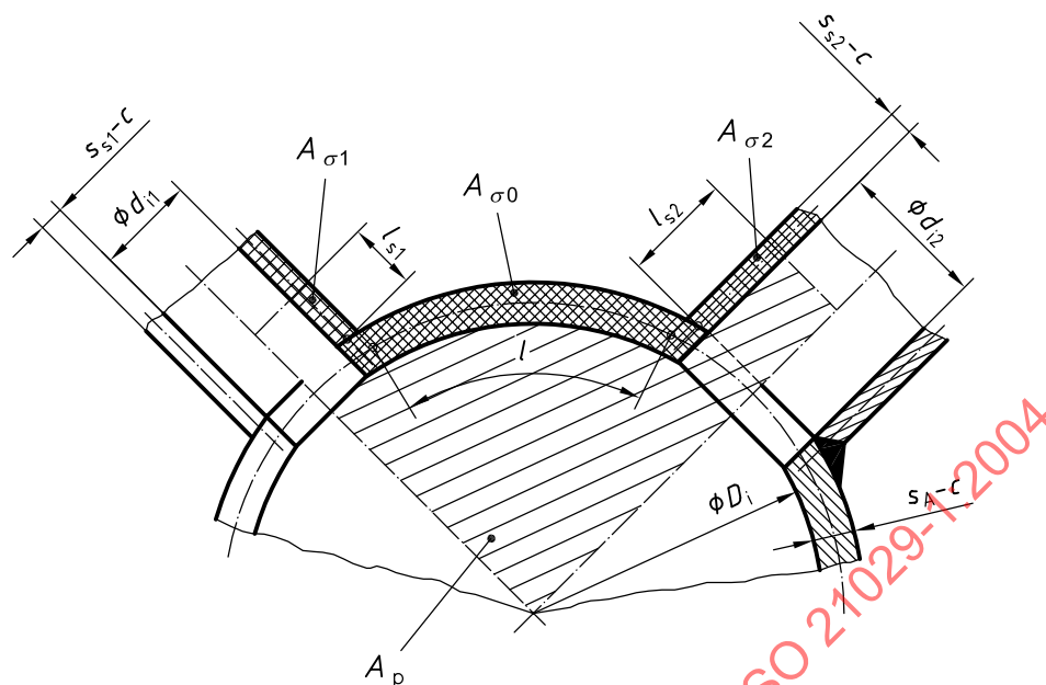
Figure 25 — Calculation scheme for adjacent nozzles in a sphere or in a circumferential direction of a cylinder
