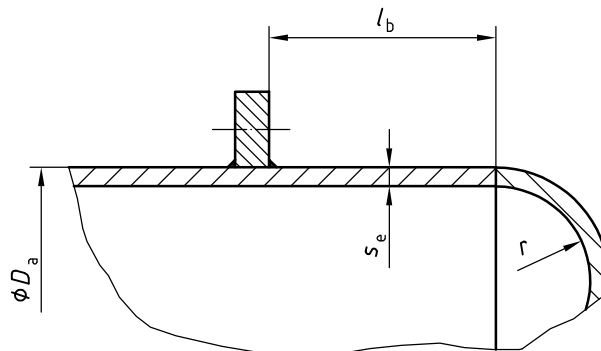
Figure 3 — Dished ends
