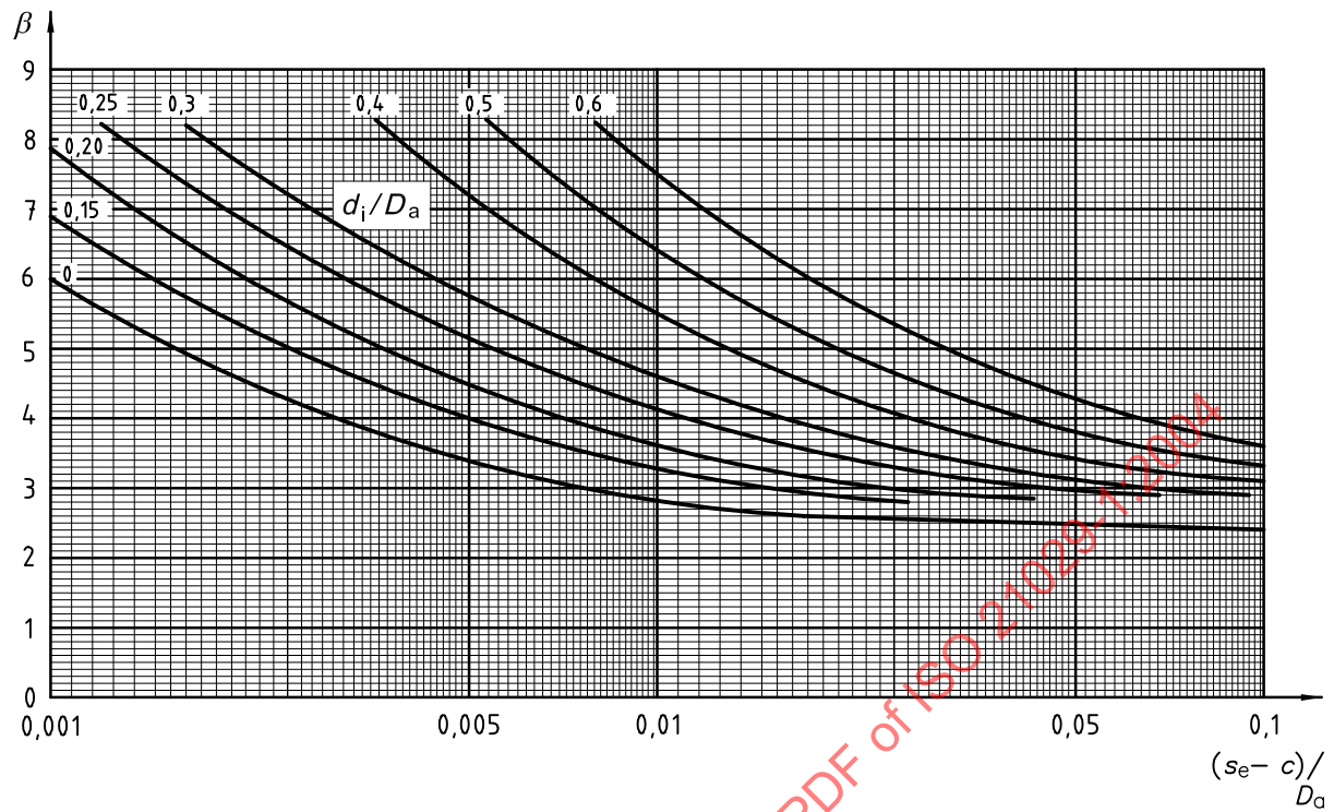
a) 10 % torispherical dished ends
