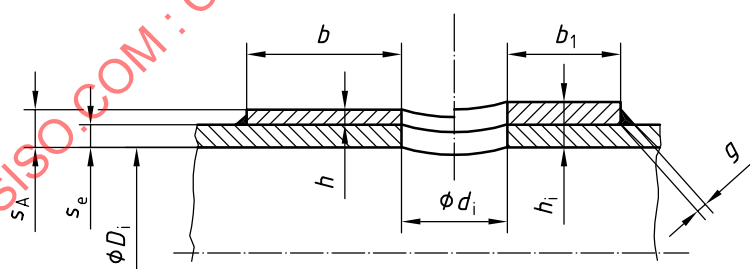
Figure 18 — Pad reinforcement
