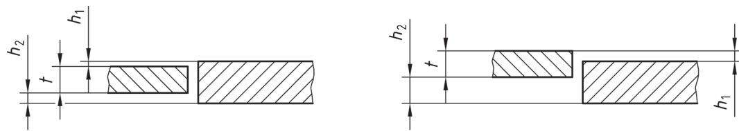
a) Seams which do not require a taper
