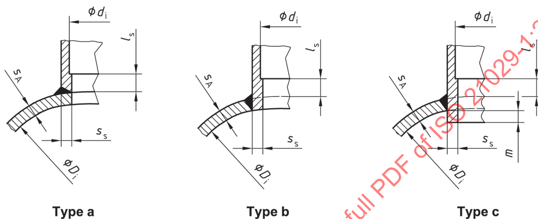
Figure 19 — Nozzle reinforcement
