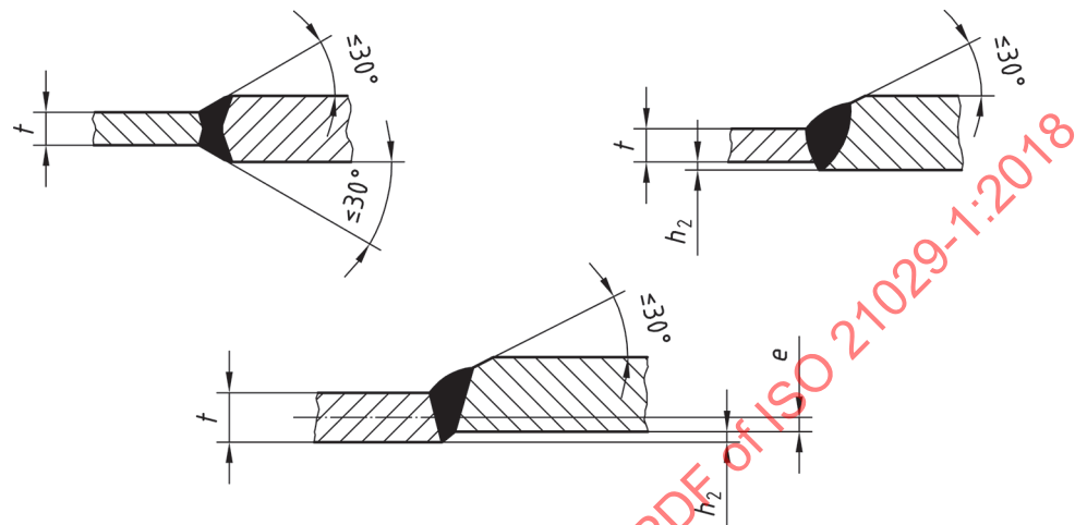
b) Seams which do require a taper
