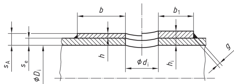
Figure 18 — Pad reinforcement
