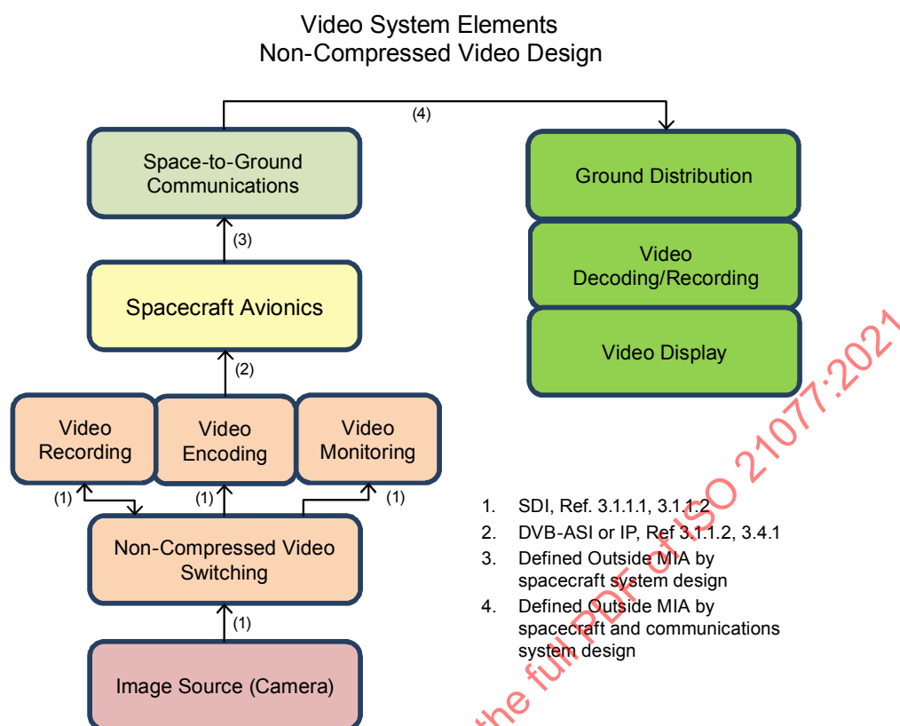
Figure 3-1: Video System Elements—Non-Compressed Video Design
