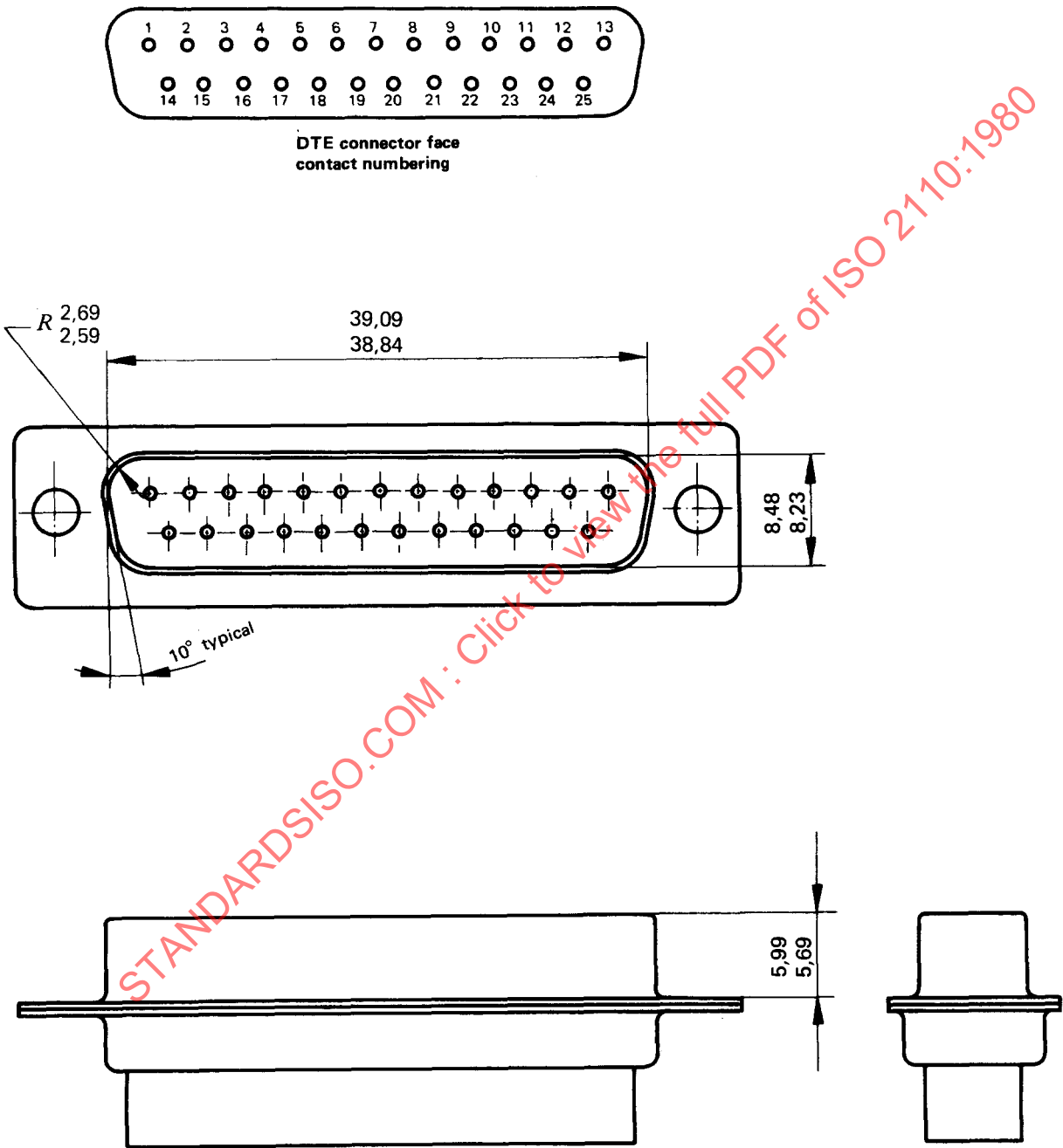
Figure 1 — DTE interface connector
