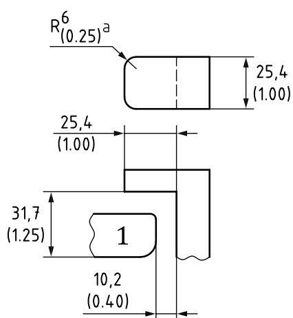
Figure 18 — Restraint condition plan view
