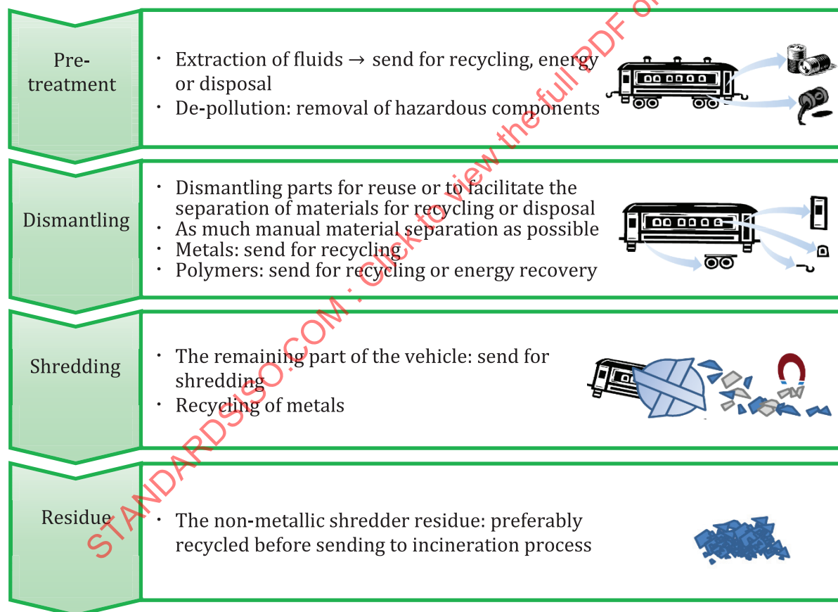
Figure 3 — Illustration of the end-of-life treatment stages for rolling stock
