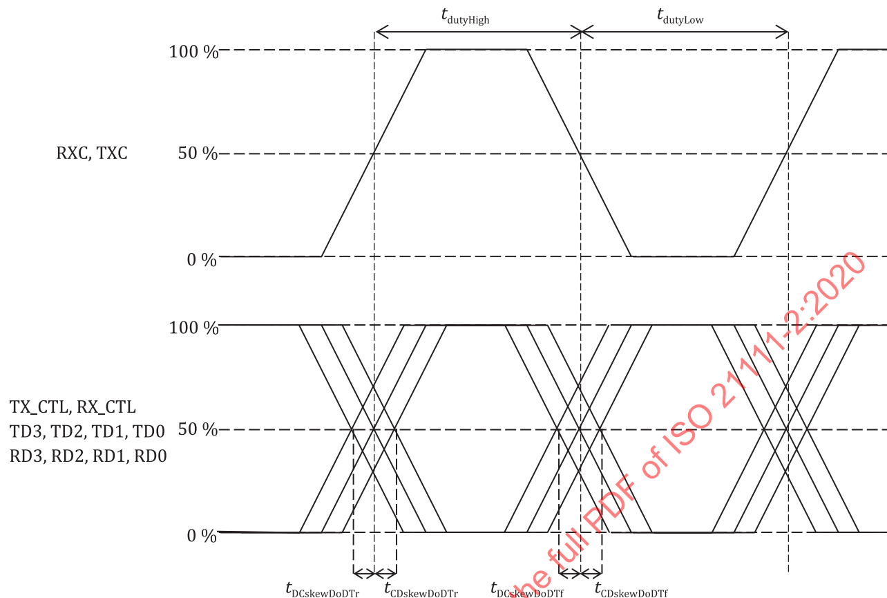
Figure 4 — Electrical signal timing parameters at source side in DoD mode
