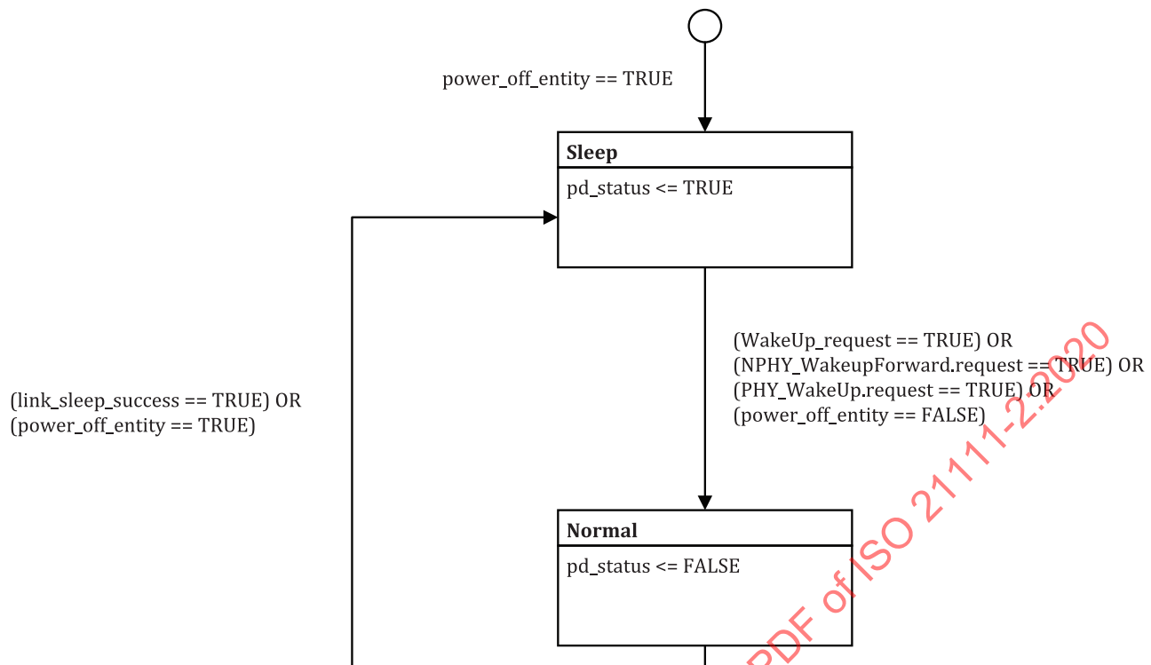
Figure 8 — Physical entity power state diagram
