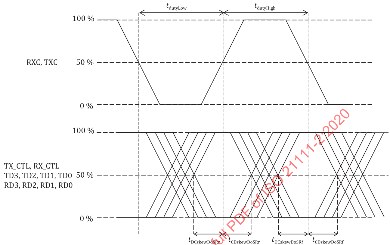
Figure 7 — Electrical signal timing parameters at destination side on DoS mode
