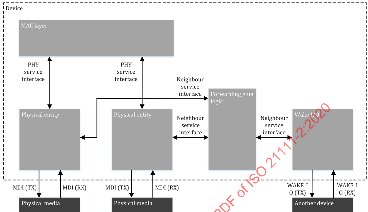
Figure 10 — Example of a device with two physical entities, wake I/O and forwarding glue logic
