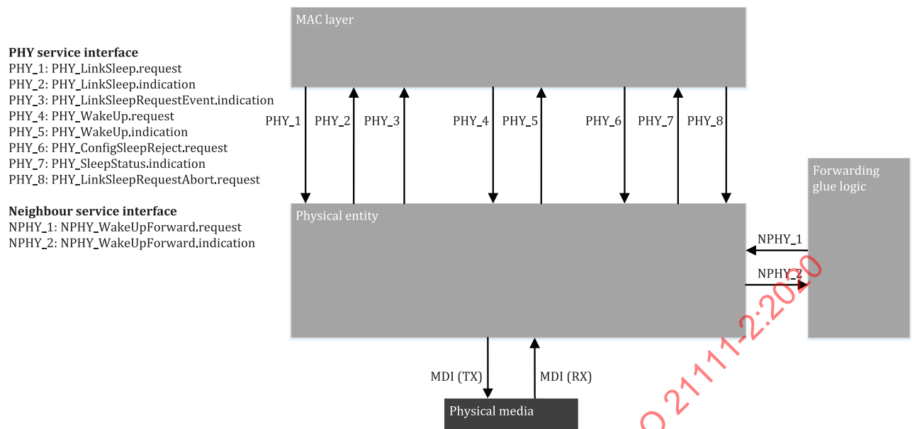
Figure 9 — Physical entity service primitives
