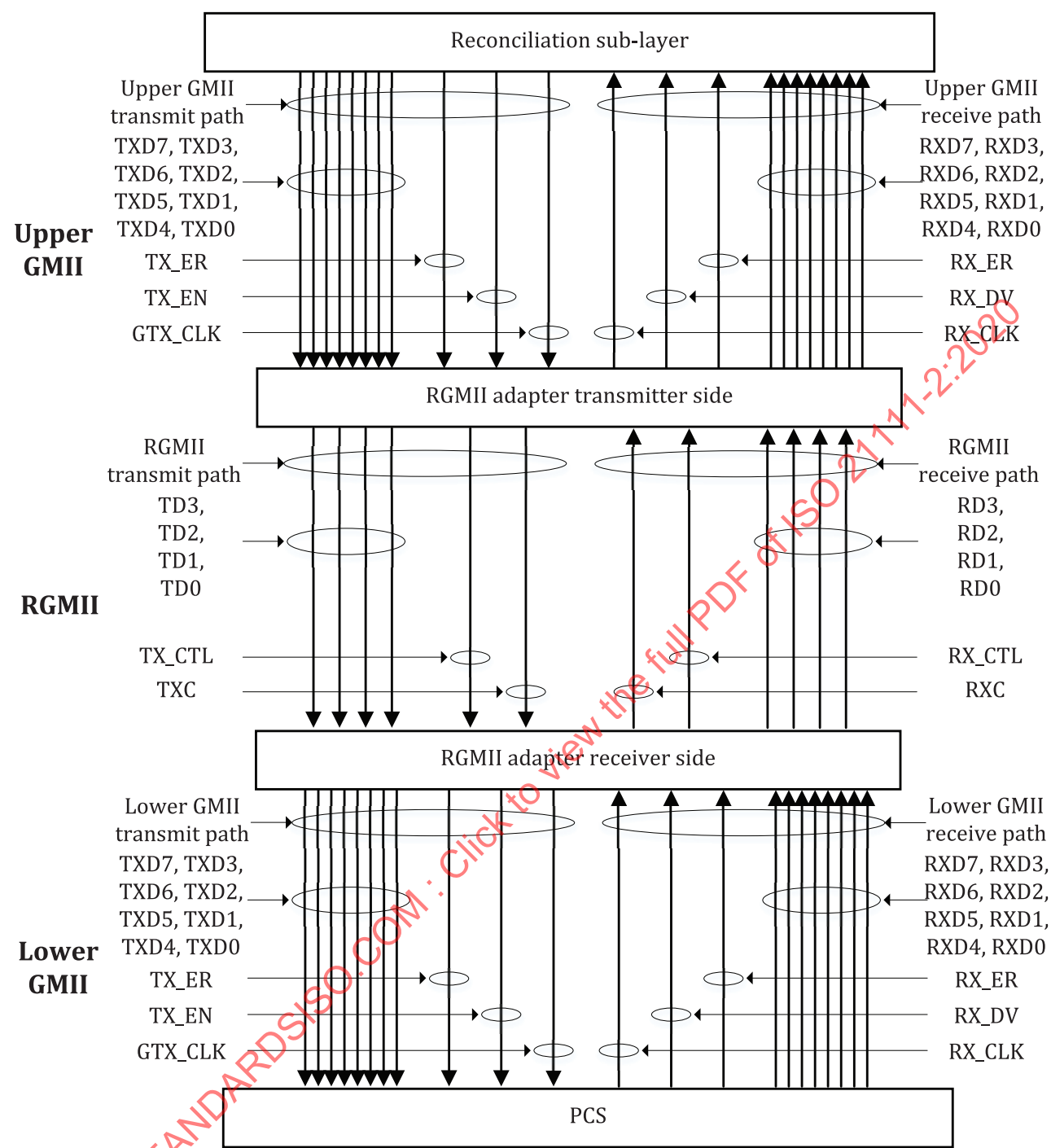
Figure 2 — RGMII architecture
