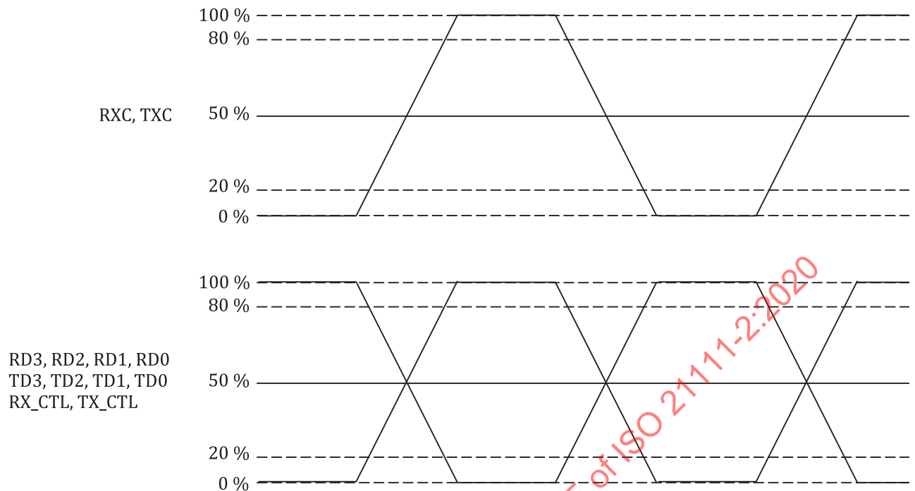
Figure 3 — RGMII electrical signal voltage level
