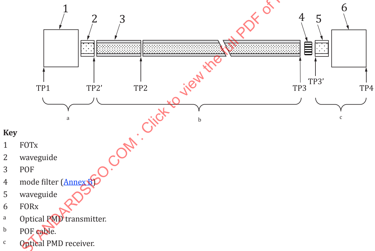
Figure 22 — Position of test points
