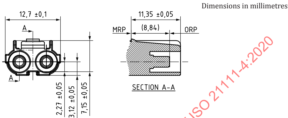
Figure 7 — Cable plug (type A)
