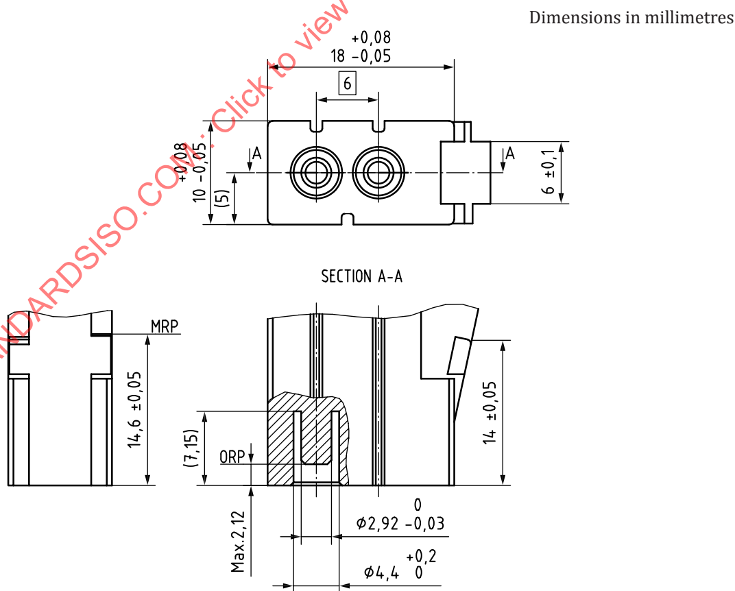
Figure 8 — Cable plug (type B)
