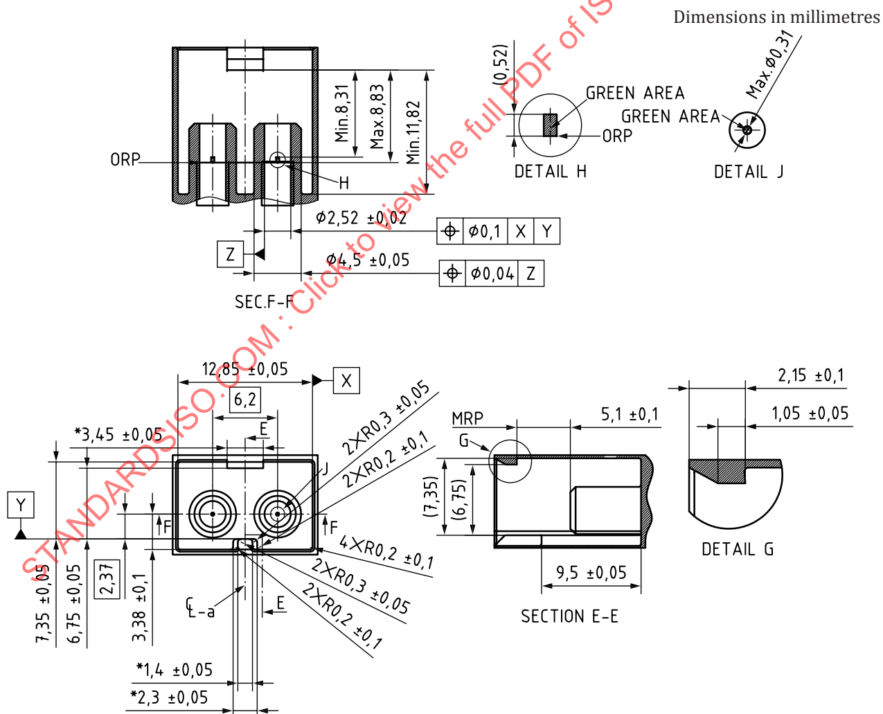
Figure 9 — Cable socket (type A)
