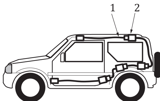
Figure 20 — Optical harness with in-line connectors
