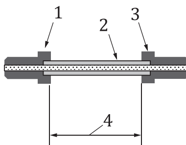
Figure 27 — Optical power pick-up system
