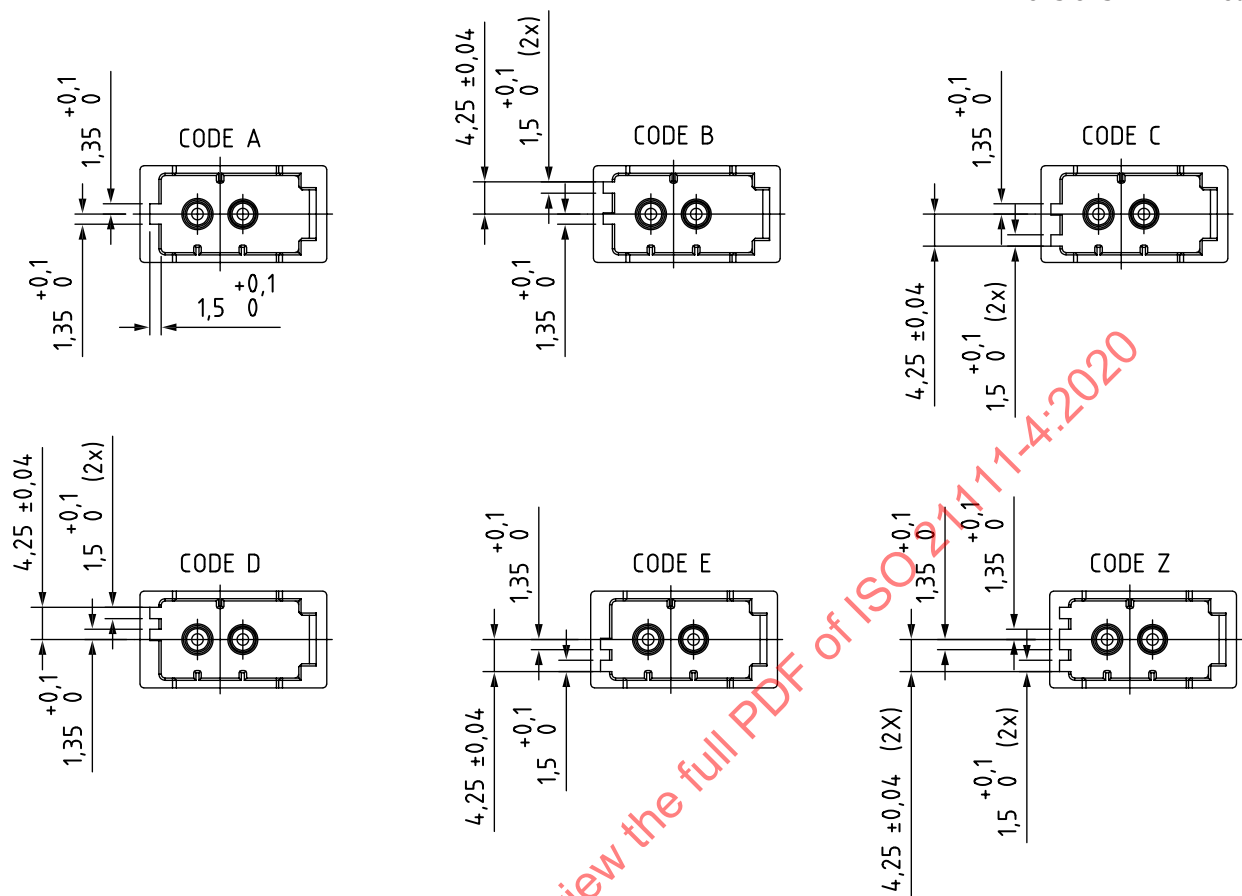
Figure 6 — Mechanical coding (type B)
