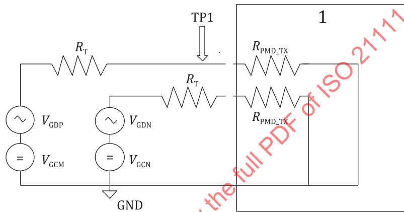
Figure 24 — 1000BASE-H transmitter electrical model and optical PMD transmitter model
