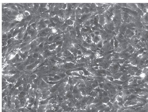
e) 25 mg/l 3,4-DCA (64 % metabolic activity) f) 12,5 mg/l 3,4-DCA (81 % metabolic activity)
