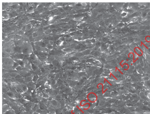
a) Negative control (100 % metabolic activity) b) Solvent control (100 % metabolic activity)
