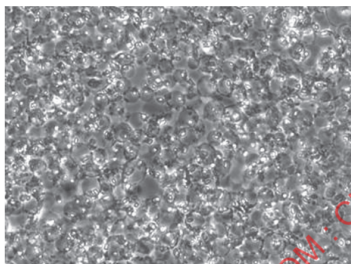
c) 100 mg/l 3,4-DCA (2 % metabolic activity) d) 50 mg/l 3,4-DCA (12 % metabolic activity)
