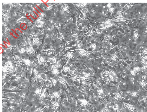
c) 100 mg/l 3,4-DCA (2 % metabolic activity) d) 50 mg/l 3,4-DCA (12 % metabolic activity)
