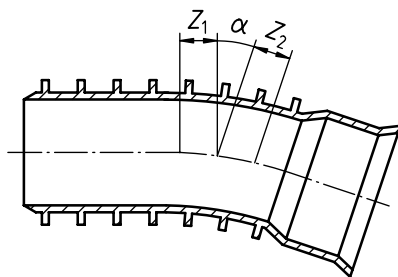
Figure 1 — Example of an unswept bend
