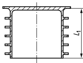
Figure 7 — Example of a plug
