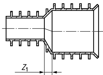
Figure 4 — Example of a reducer
