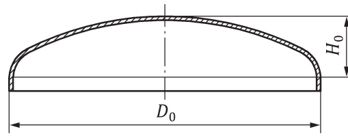
Figure B.2 — Torispherical end equivalent height
