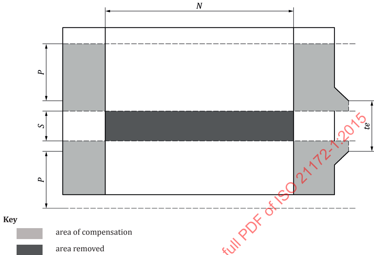
Figure 4 — Opening compensation
