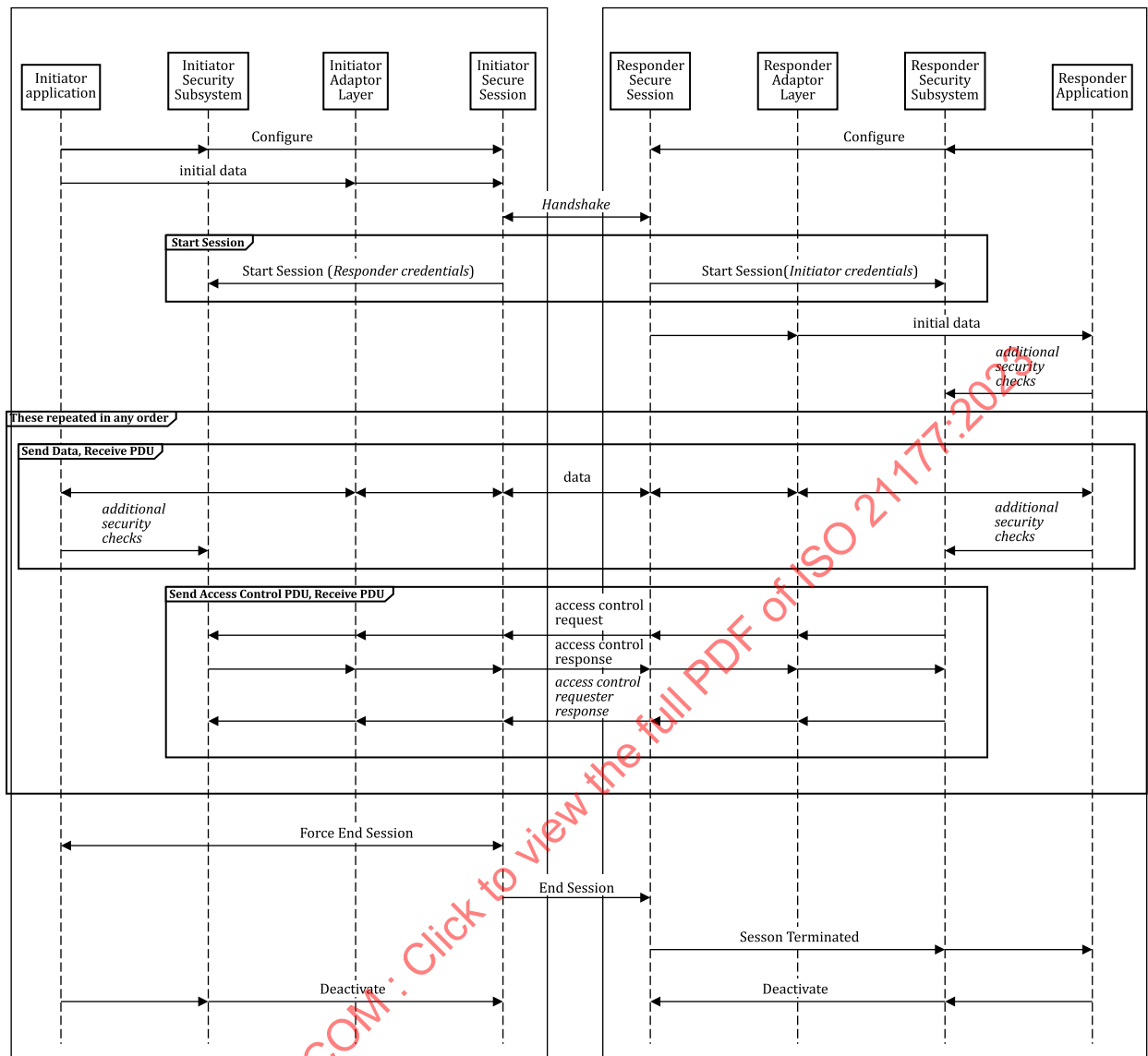
Figure 27 — Sequence diagram for complete secure session example
