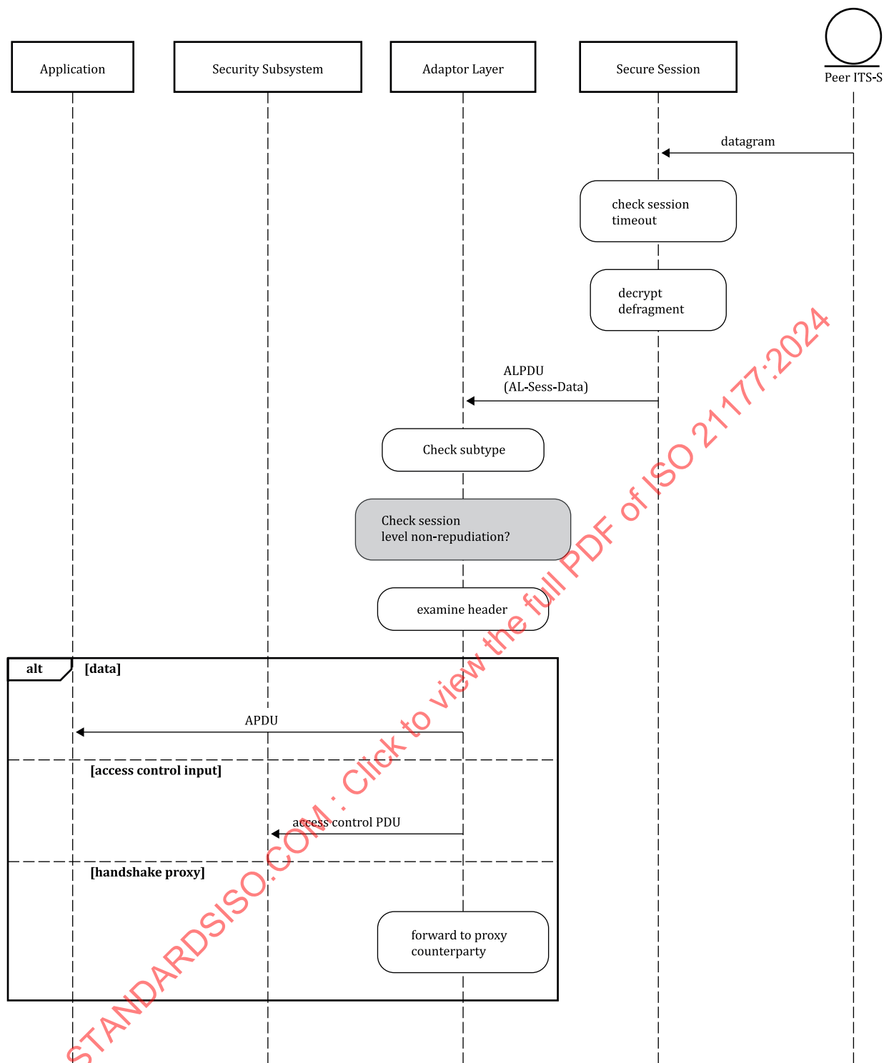
Figure 16 — Sequence diagram for incoming datagrams (overview)
