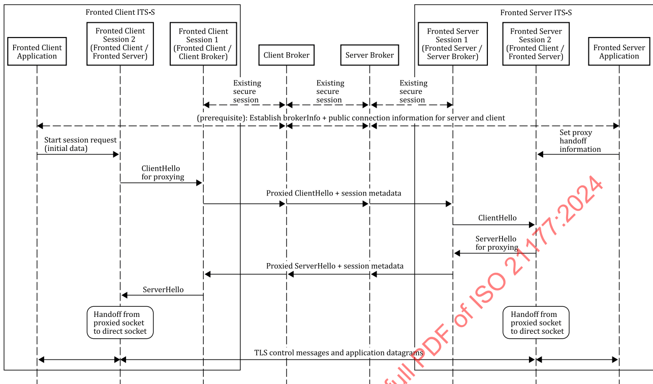
Figure 19 — Overview sequence diagram for secure connection brokering
