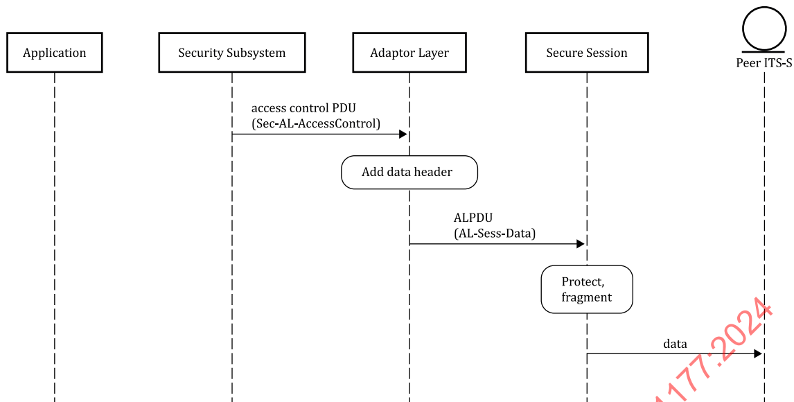
Figure 15 — Sequence diagram for sending access control PDU
