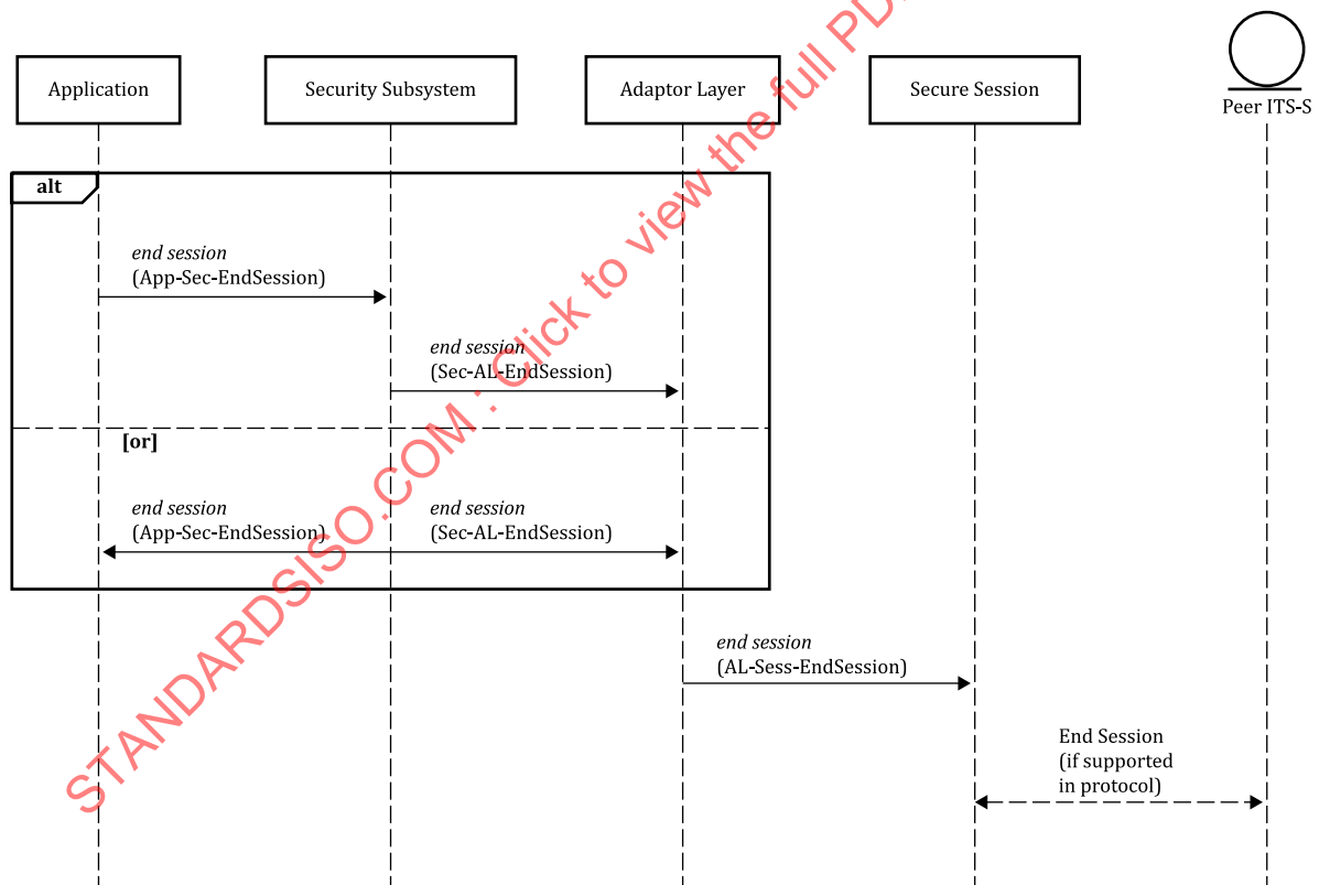
Figure 24 — Sequence diagram for Force End Session
