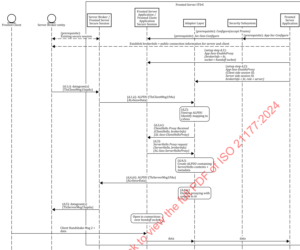
Figure 23 — Sequence diagram for secure connection brokering operations on the fronted server
