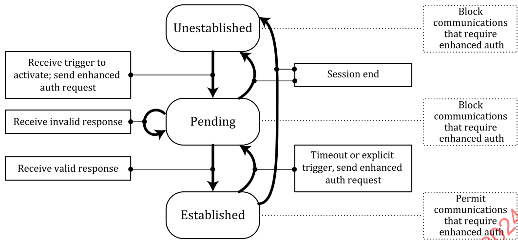
Figure 28 — Informal state machine for the enhanced authentication module
