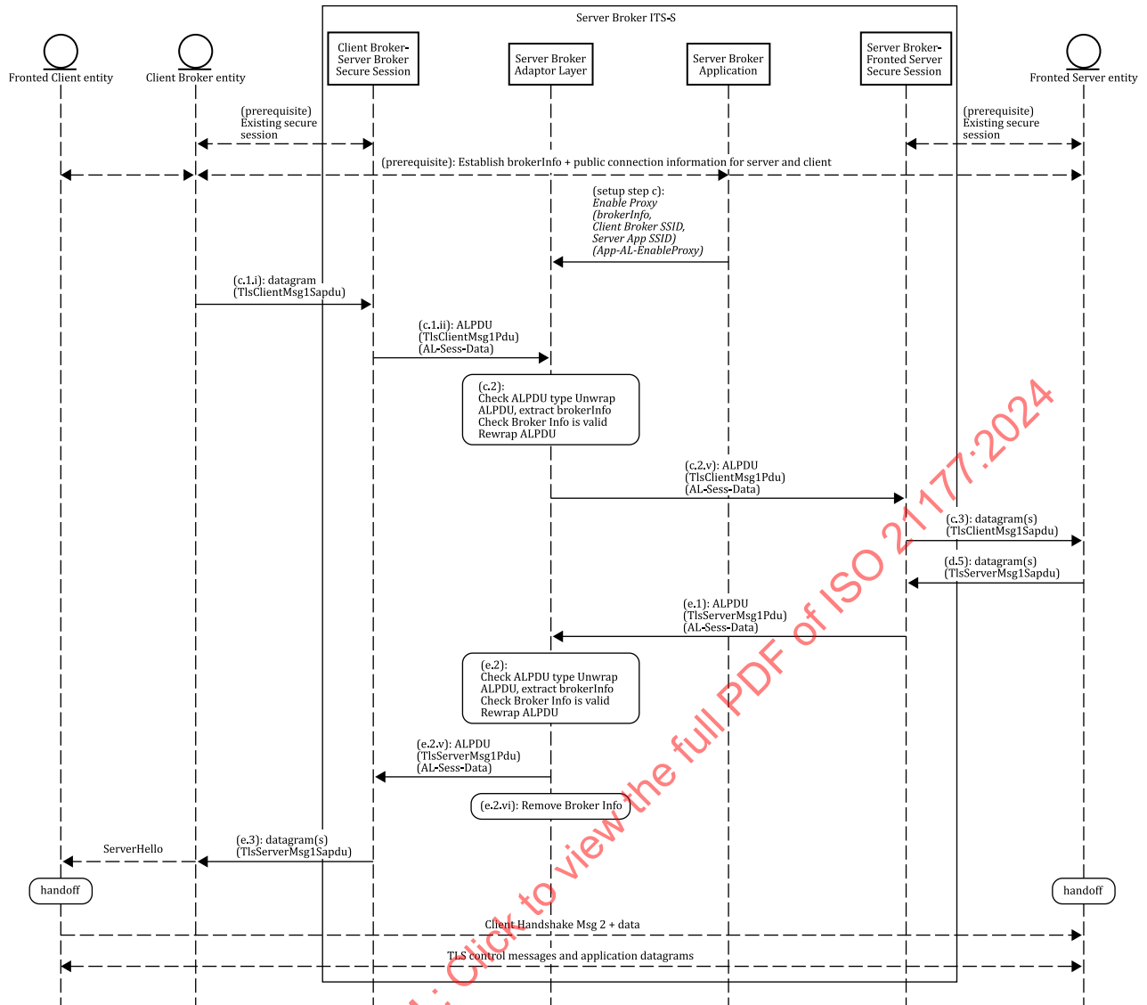
Figure 22 — Sequence diagram for secure connection brokering operations on the server broker
