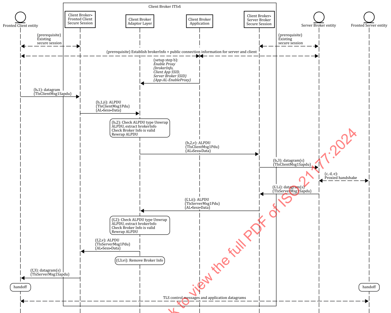
Figure 21 — Sequence diagram for secure connection brokering operations on the client broker
