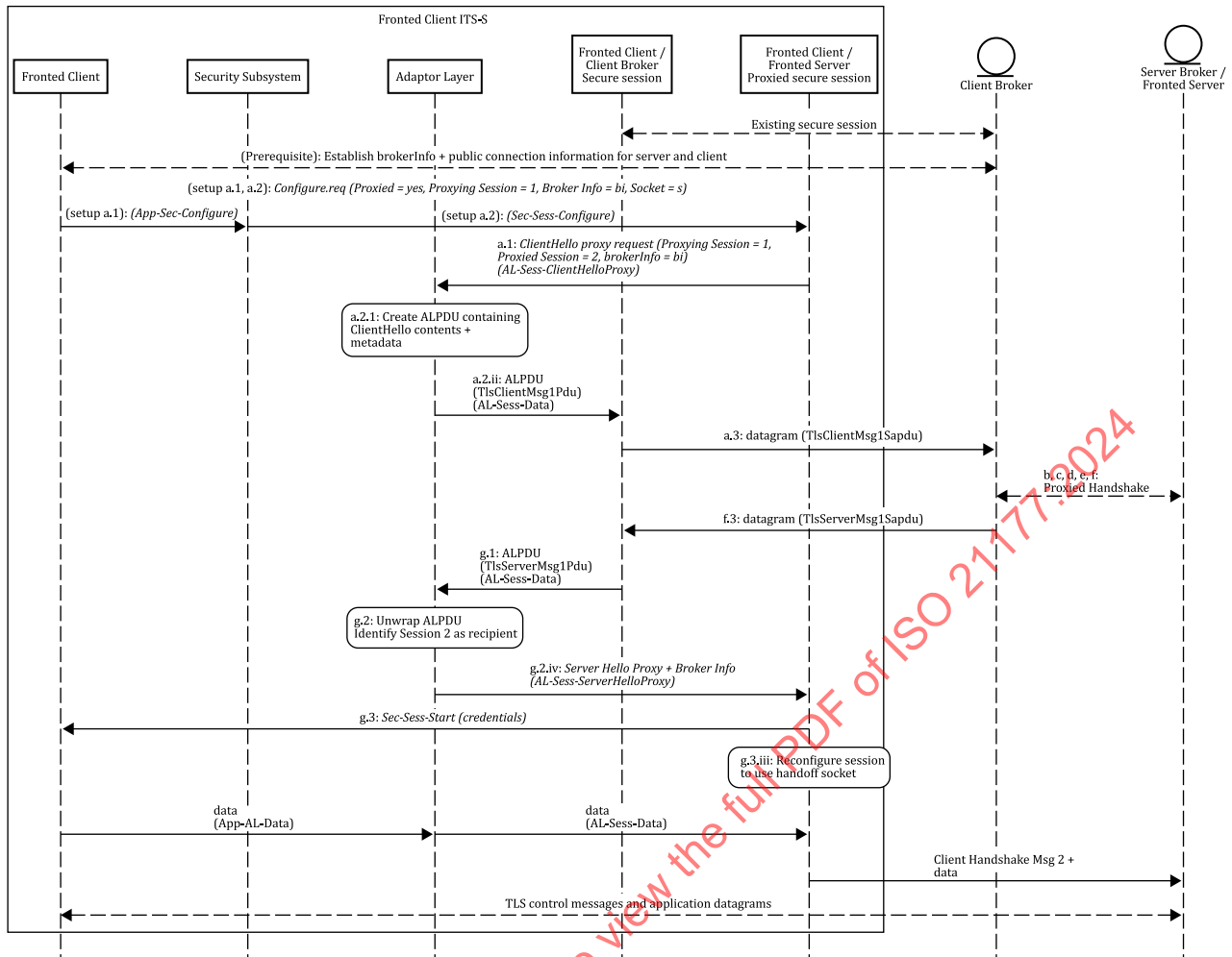
Figure 20 — Sequence diagram for secure connection brokering operations on the fronted client
