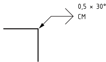
Figure 34 — Chamfer maximum material boundary specification
