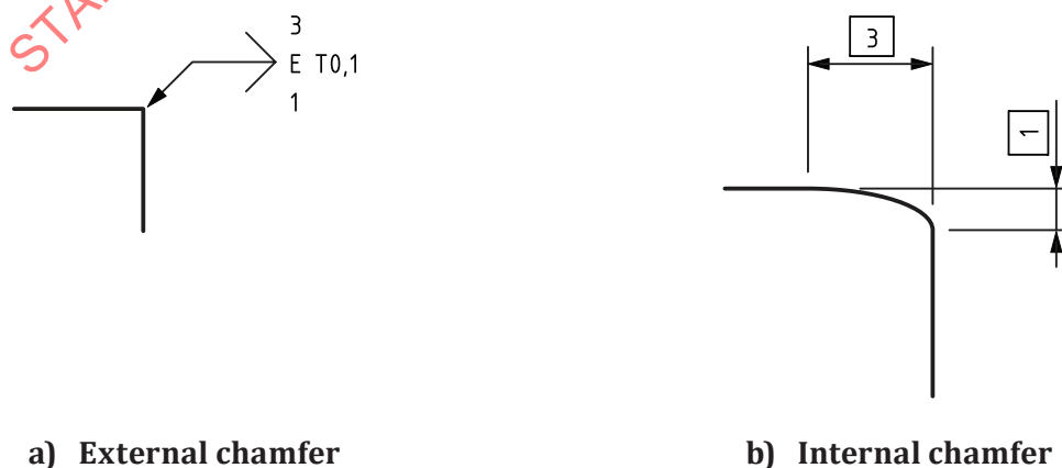
Figure 44 — Elliptical profile specification
