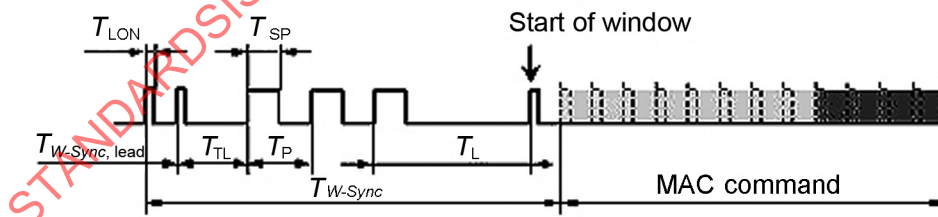
Figure 9 — Window synchronisation ( W -Sync)
