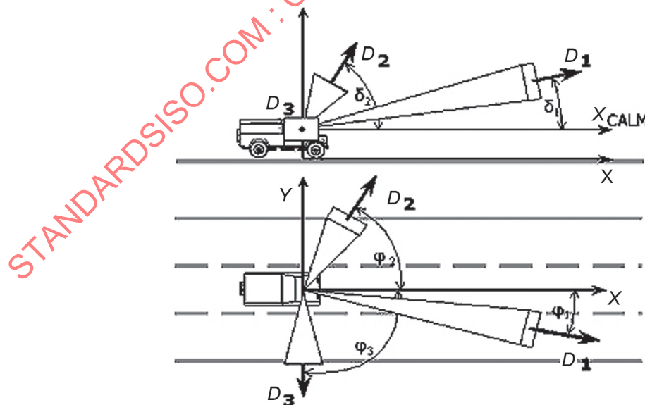
Figure D.1 — Example of multi beam antenna
