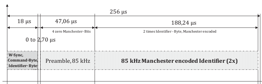
Figure 2 — Wake-up signal
