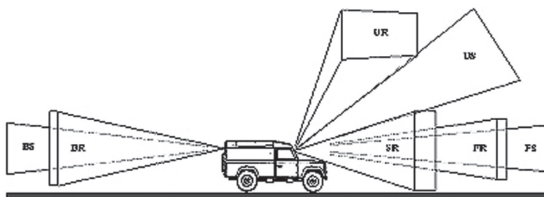
Figure D.2 — Example of side view of communication zones
