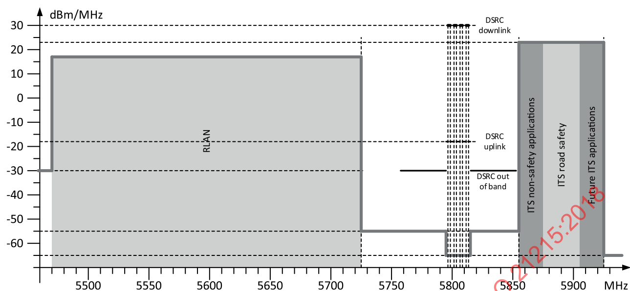
Figure F.1 — Power spectrum density for Europe
