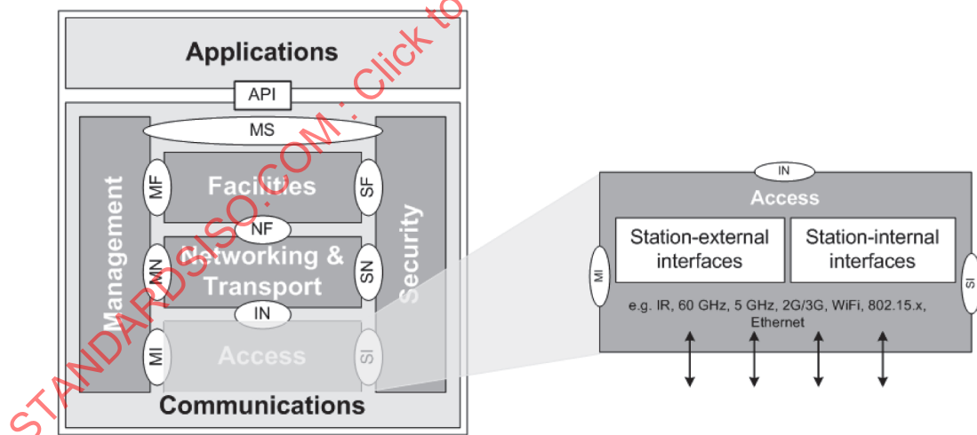
Figure 16 — ITS-S reference architecture - ITS-S access layer
