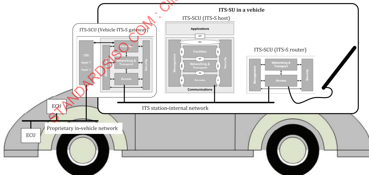
Figure A.1 — ITS-SU in a vehicle (V-ITS-SU)
