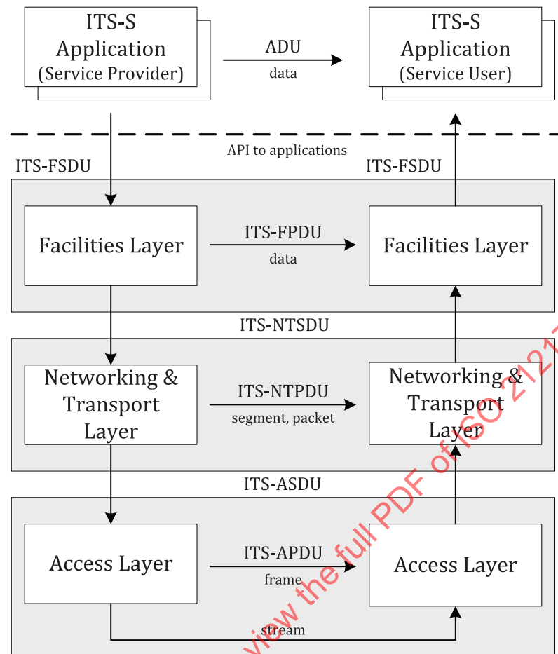
Figure 16 — OSI data unit transfer in an ITS station
