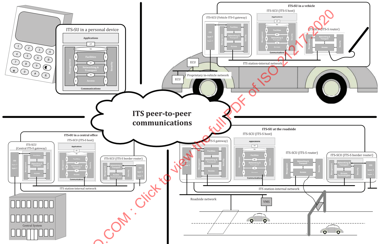
Figure 29 — Typical implementations of ITS station units
