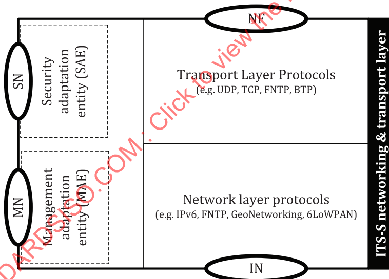
Figure 23 — Elements of the ITS-S networking and transport layer
