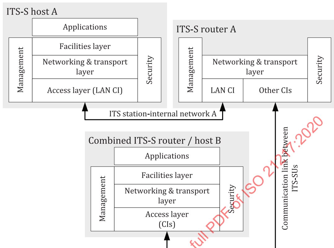
Figure 19 — Implementation architecture III.
