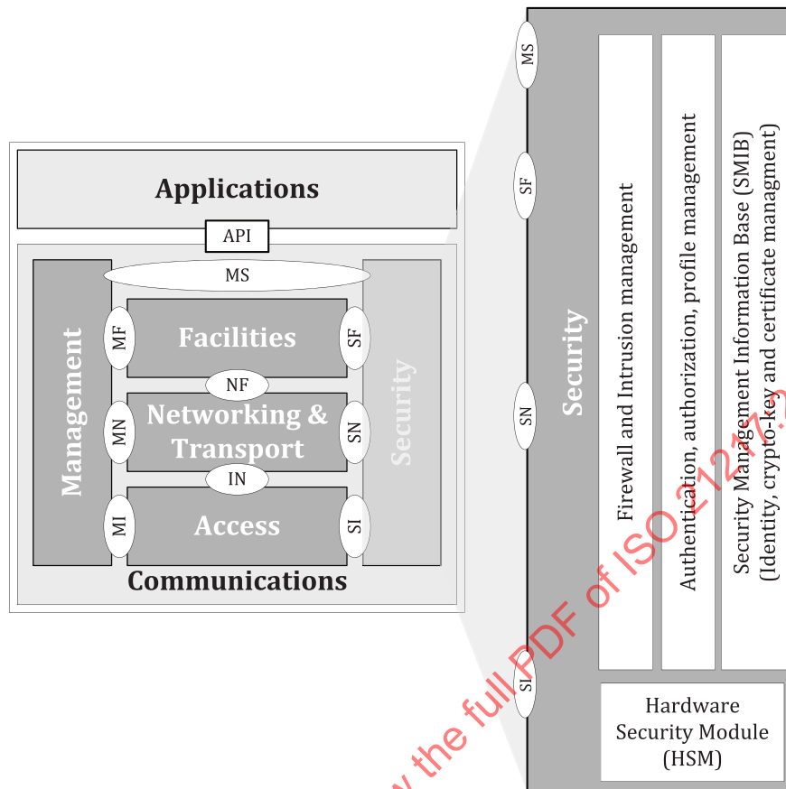
Figure 27 — ITS-S security entity as part of the ITS-S reference architecture
