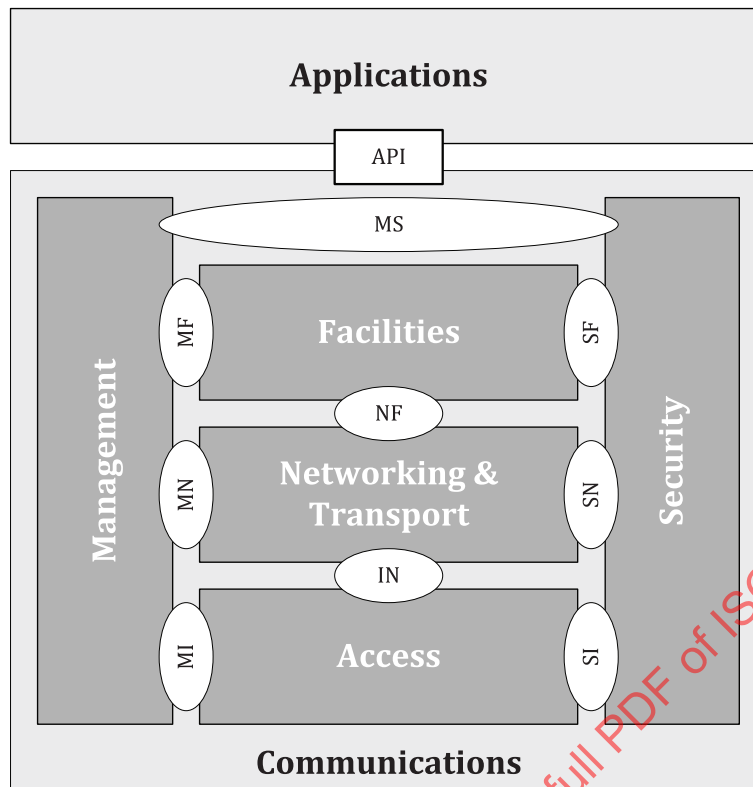
Figure 13 — Simplified ITS-S reference architecture
