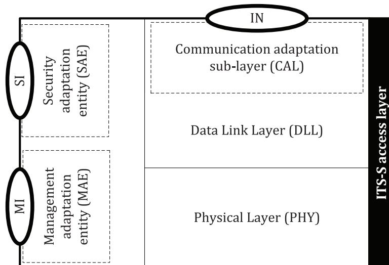
Figure 21 — Elements of the ITS-S access layer
