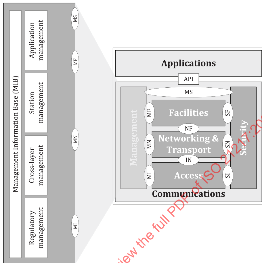
Figure 26 — ITS-S reference architecture — management entity
