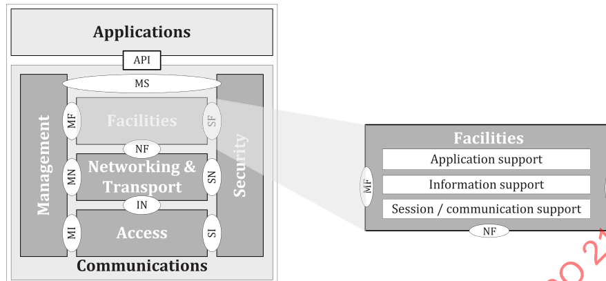
Figure 24 — ITS-S reference architecture — ITS-S facilities layer
