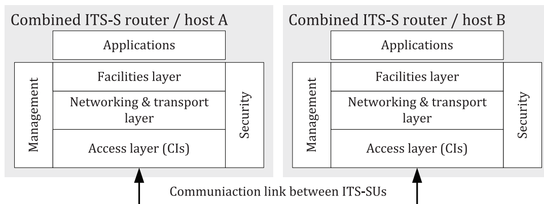
Figure 17 — Implementation architecture I
