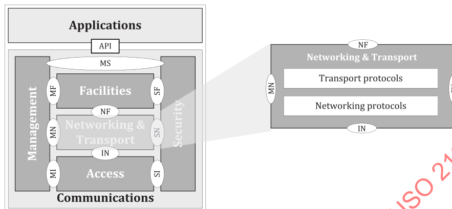
Figure 22 — ITS-S reference architecture — ITS-S networking and transport layer
