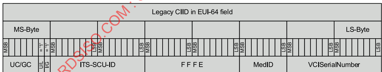
Figure C.3 — Encapsulation of identifiers specific to ITS
