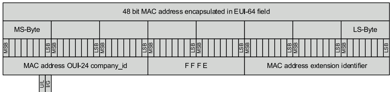
Figure C.2 — Encapsulation of 48-bit MAC address in EUI-64 field[20]
