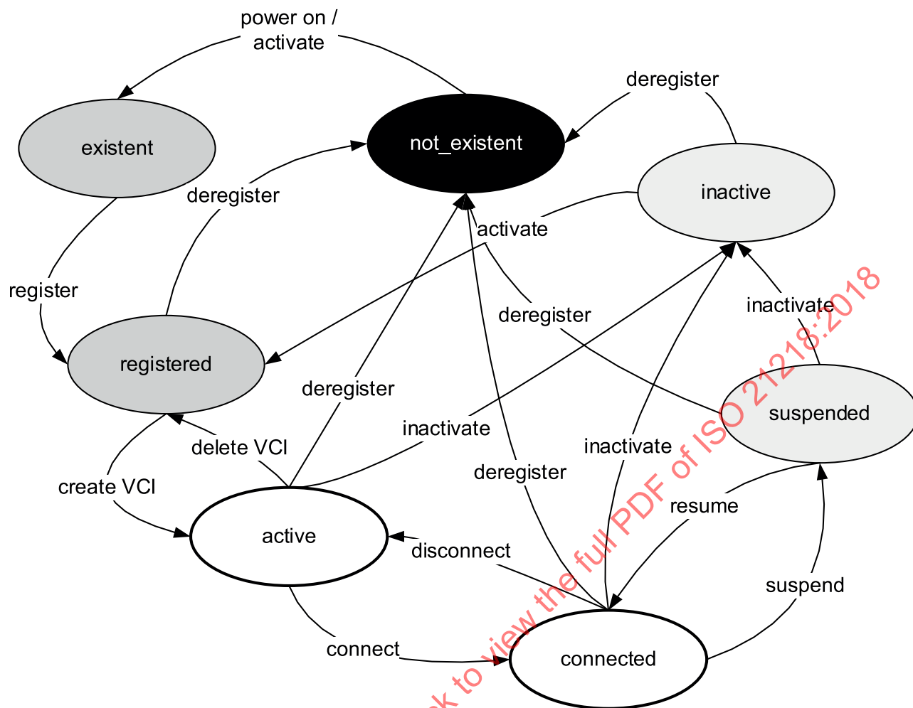
Figure 4 — CI state machine
