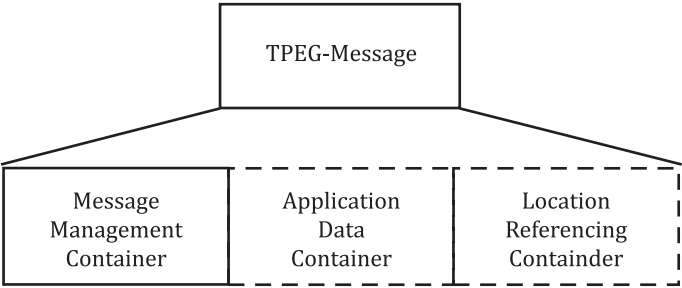
Figure 1 — Composition of TPEG messages
