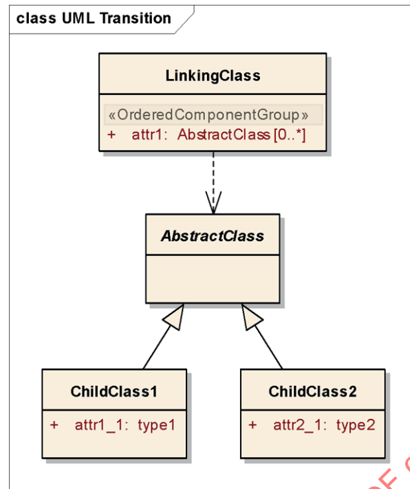
Figure 6 — Linking of abstract class
