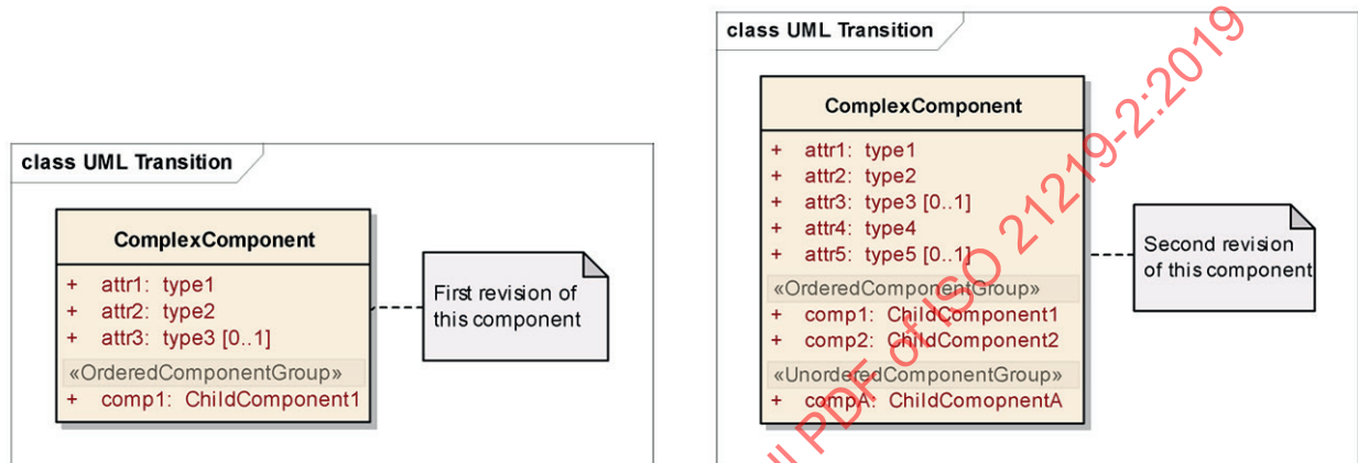
Figure 7 — Extending a TPEG component in a backwards compatible way
