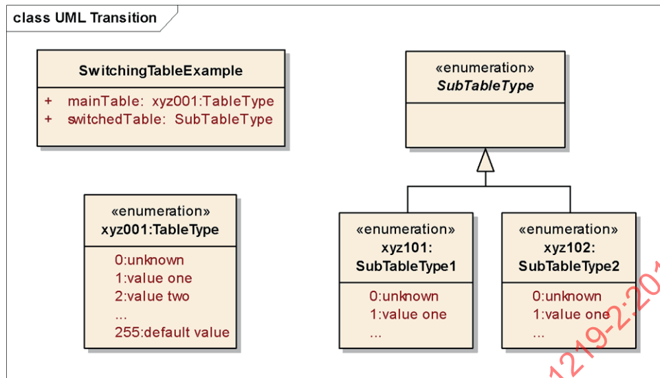
Figure 5 — TPEG Switching Table concept
