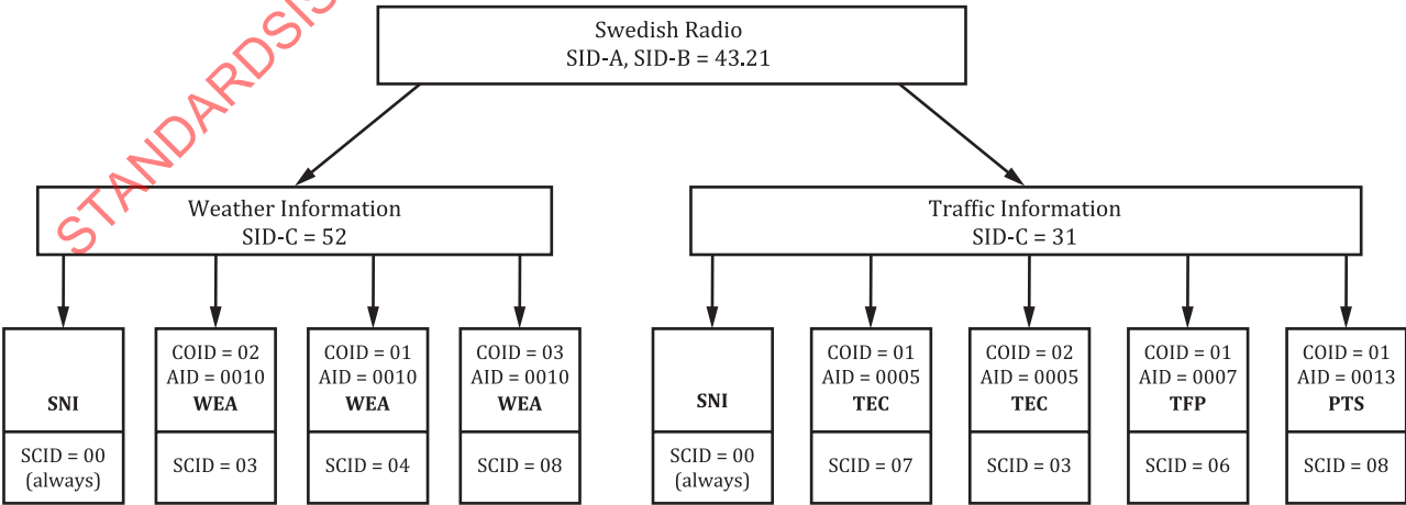
Figure 4 — Example of service allocation on a wideband bearer
