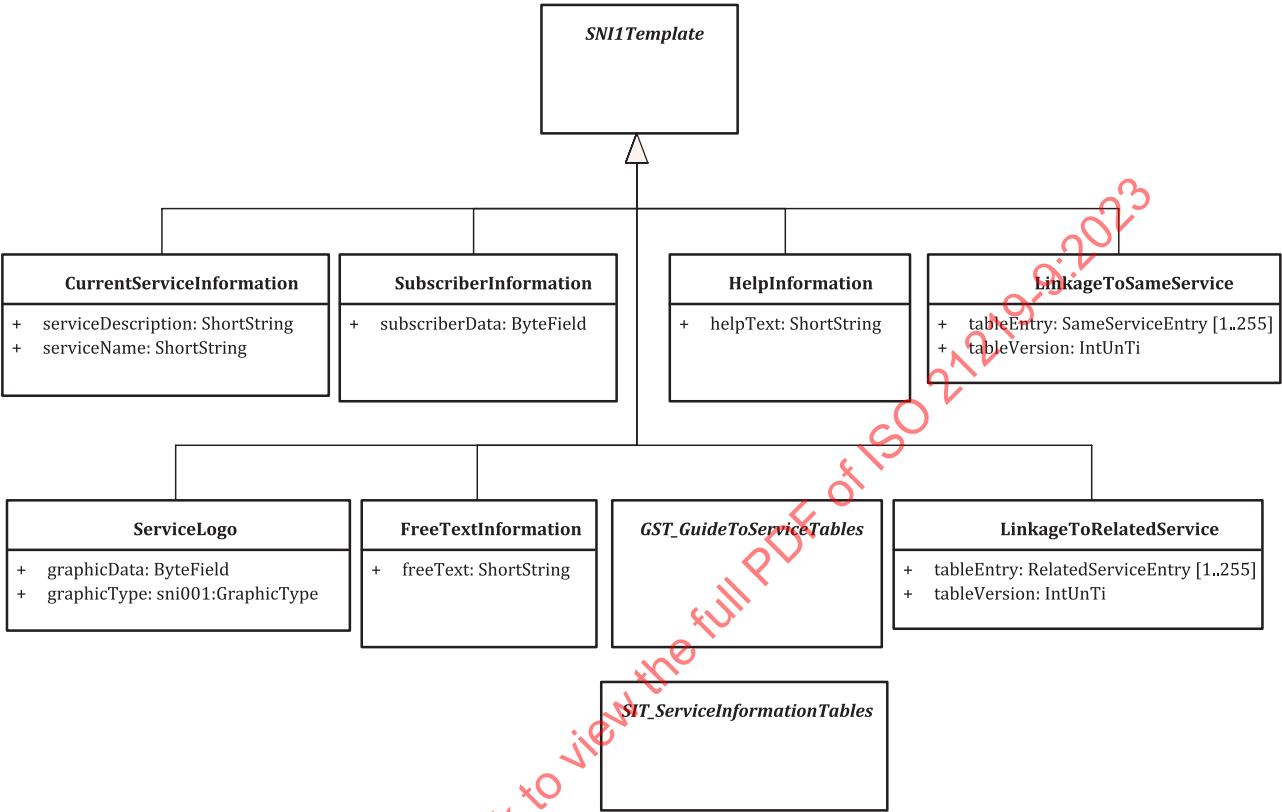
Figure 6 — SNI message structure
