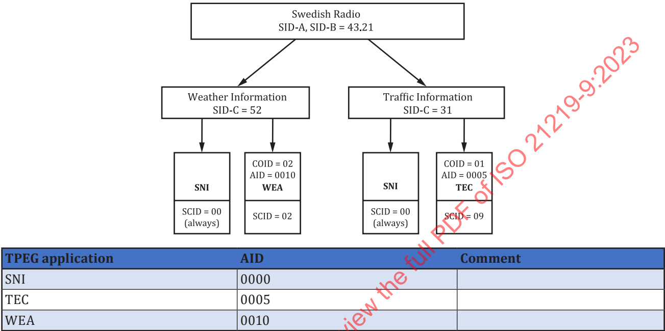
Figure 5 — Example of service allocation on a narrowband bearer
