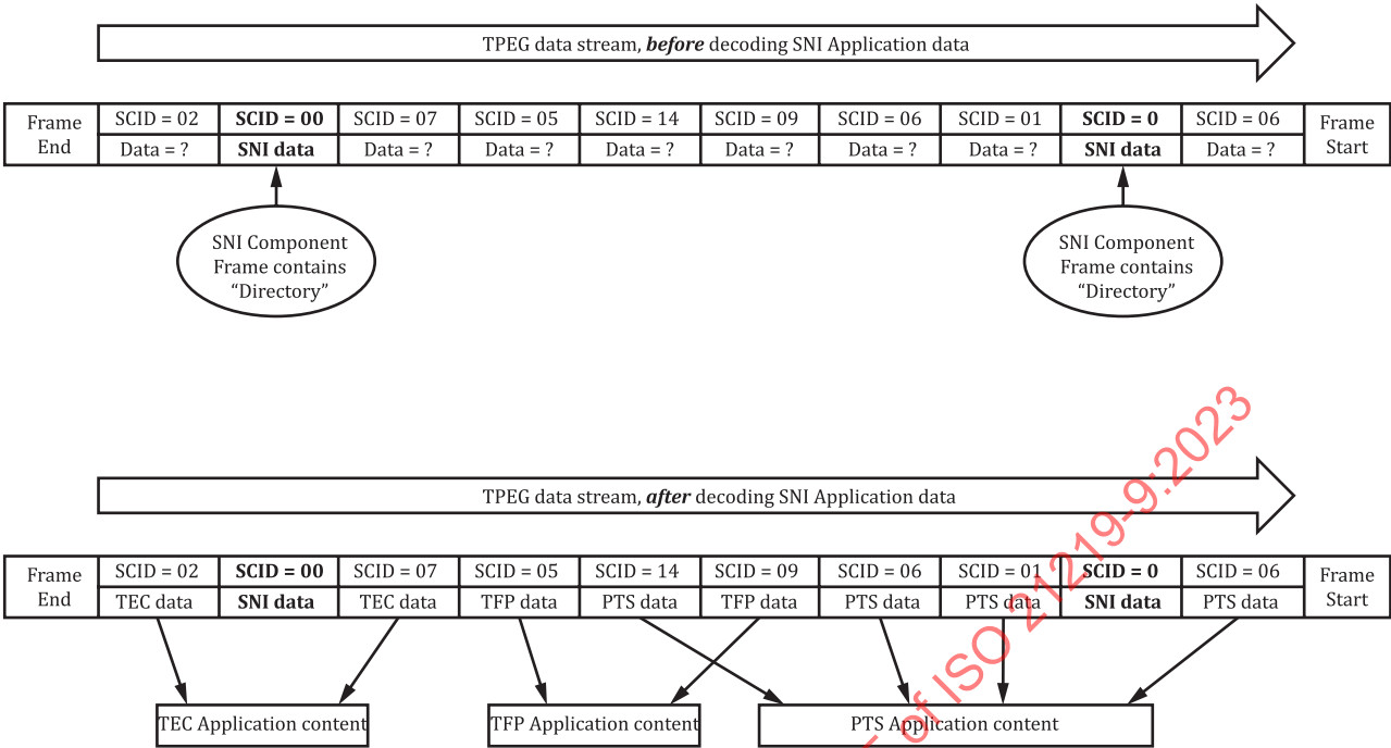
Figure 3 — Example of the TPEG-SNI application in a TPEG data-streamConcept of allocating services
