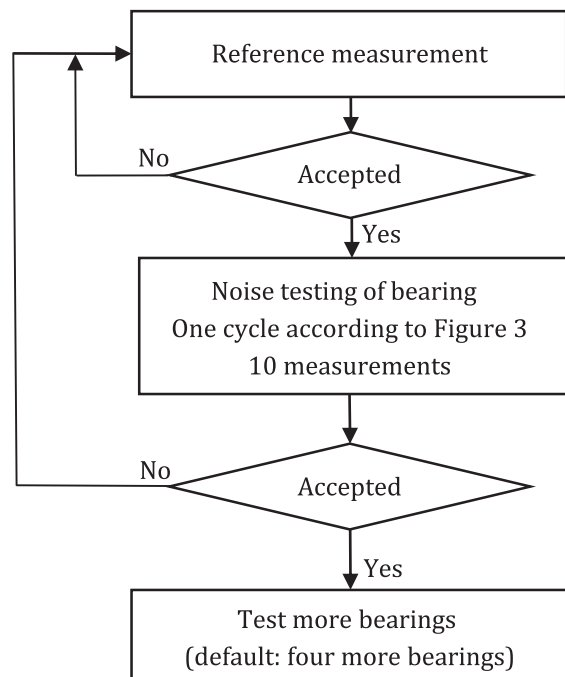
Figure 2 — Flow chart of grease noise assessing BQ+
