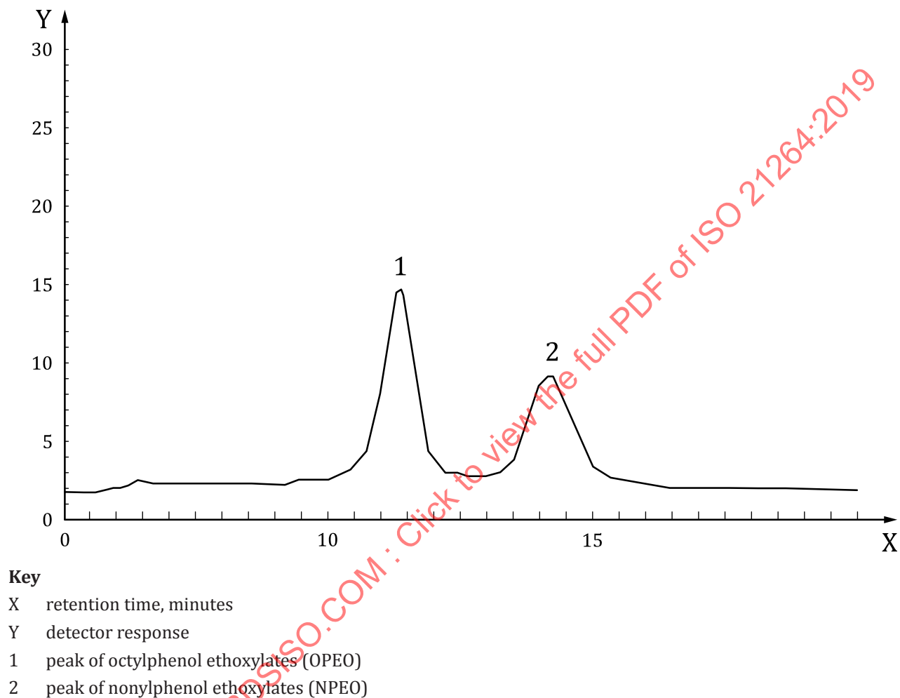
Figure A.1 — Chromatogram of OPEO and NPEO from HPLC
