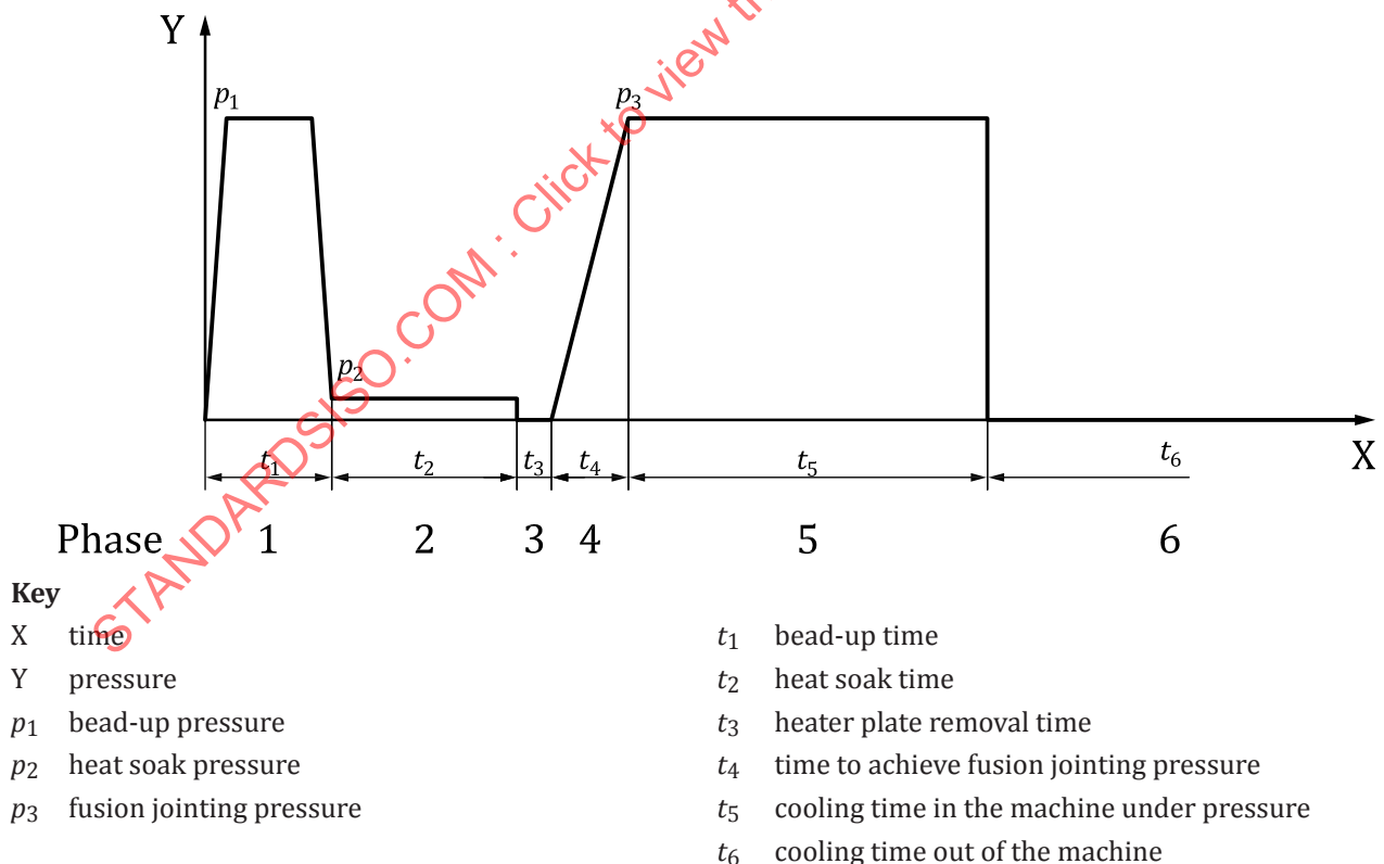
Figure 3 — Single high-pressure fusion joining cycle
