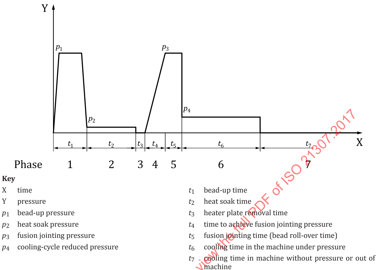
Figure 2 — Dual low-pressure fusion jointing cycle
